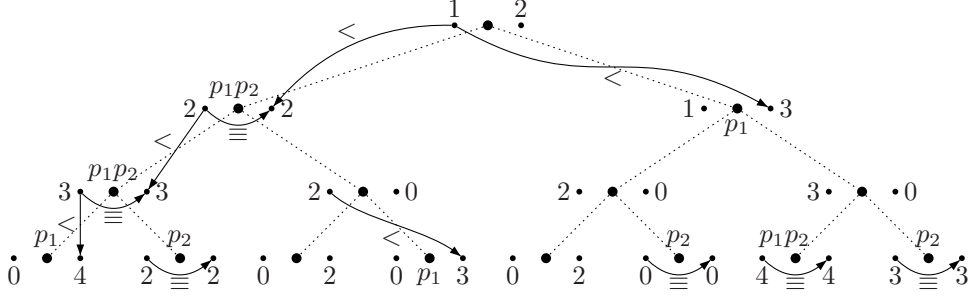
Figure 1: The (\mathbb{N}, <, \equiv) -constraint 2-tree \mathbb{T} from Example 29, the Kripke 2-tree \mathbb{T}^a , and the structure \mathcal{G}_{\mathbb{T}^a} .
