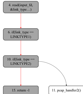
(c) The path followed by a seed that matches neither LINKTYPE1 nor LINKTYPE2.
