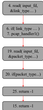
(b) The path followed by a seed that matches LINKTYPE1 but mismatches PACKET1.
