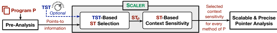
Figure 5: Overview of the SCALER framework.
