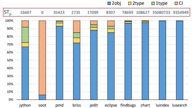
Figure 7: The ST_p value (on top of each bar) computed by SCALER for each program and the distribution of different kinds of context-sensitivities selected according to each ST_p .
