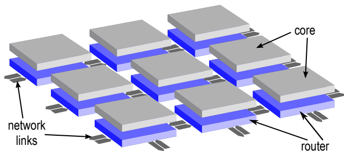
Fig. 1. A multicore system simulated by HORNET. The gray tiles (top) can be trace-driven packet injectors, cycle-level MIPS core models, or threads of an executable run under Pin; the blue tiles (bottom) are cycle-level models of a flit-based virtual-channel wormhole router. While the illustration shows a 2D mesh, HORNET can construct a system with any interconnect geometry.
