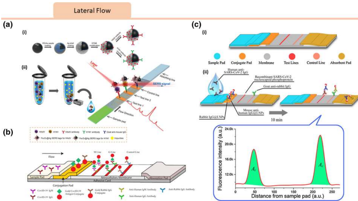
FIGURE 8. Viral Lateral Flow Sensors: (a) Schematic of antibody-modified \text{Fe}_3\text{O}_4@Ag magnetic tags and magnetic SERS strip for respiratory viruses detection. (i) \text{Fe}_3\text{O}_4@Ag magnetic tags are modified with dye molecules (DTNBs) and capture antibodies acting as capturing and enhancing substrate while dual-labeled DTNB molecules generating SERS signals. (ii) The magnetic SERS-LFIA system components and operating procedure. 80 Reprinted with permissions from ACS Appl. Mater. Interfaces 2019, 11, 21, 19495–19505. Copyright (2019) American Chemical Society. (b) Schematic of SARS-CoV-2 IgM-IgG combined antibody test. Two mouse anti-human monoclonal antibodies (anti-IgG and anti-IgM) are coated on different test lines, while surface antigen from SARS-CoV-2 is conjugated to colloidal gold nanoparticles on conjugation pads. 35 This is an open access article distributed under the terms of the Creative Commons CC BY. (c) Schematic of lanthanide-doped nanoparticles-based lateral flow immunoassay (LFIA). (i) LFIA strips components. (ii) Analytical procedure: lanthanide-doped polystyrene nanoparticles (LNPs) are captured at the test and control line, where fluorescence at excitation and emission wavelengths of 365 and 615 nm is read. Their ratio determines the anti-SARS-CoV-2 IgG concentration in the sample. 14 This figure is reused with permission from ACS and the article can be accessed here: https://pubs.acs.org/doi/10.1021/acs.analchem.0c00784 .
