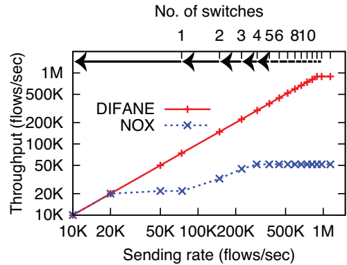
Figure 9: Throughput comparison of DIFANE and NOX.
