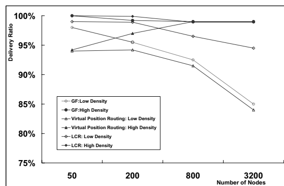
Figure 7. Comparison of Logical Coordinate Routing Schemes
