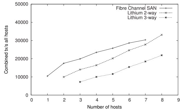
Figure 8: PostMark Scalability. Total transactions per second across all hosts, with 4 VMs per host for a varying number of hosts of Lithium in 2-way and 3-way replicated scenarios, and for a mid-range Fibre Channel storage array.
