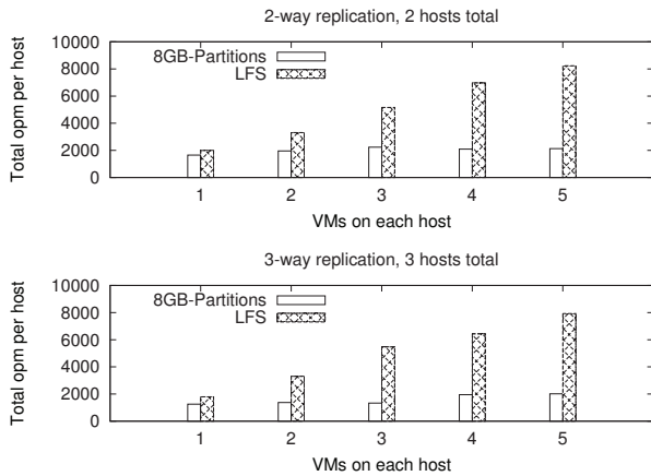
Figure 6: Performance of the DVD Store 2 OLTP benchmark in two- and three-host fully replicated scenarios.
