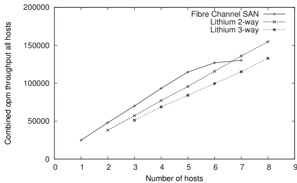
Figure 7: DVDStore2 Scalability. This graph shows the total orders per minute across all hosts, with 4 VMs per host for a varying number of hosts of Lithium in 2-way and 3-way replicated scenarios, and for a mid-range Fibre Channel storage array.
