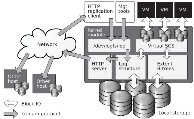
Figure 1: The components of Lithium on each host. VMs access the Lithium kernel module inside ESX through a virtual SCSI interface, and the user space replication agent and management tools append to the log through a special device node.
