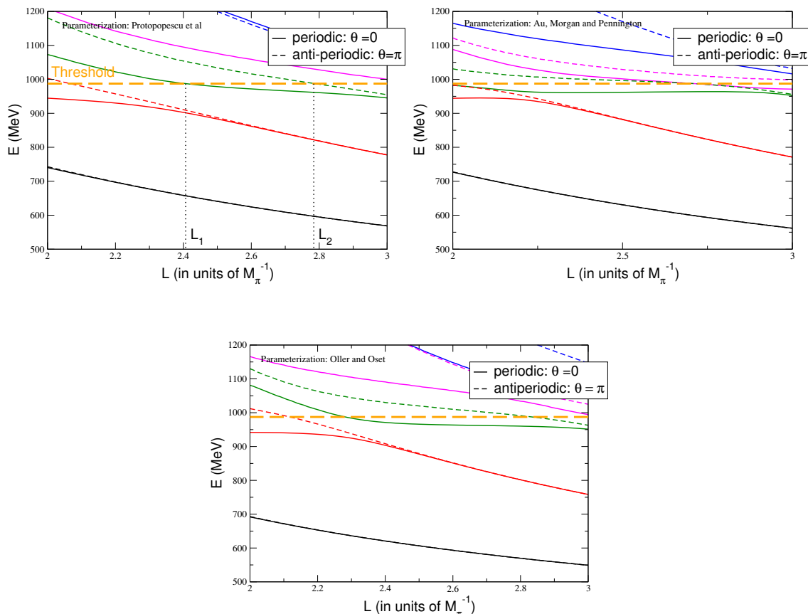
Figure 1. Energy levels E_n , n = 1, 2, \dots of the two-pion states in a finite box. Solid lines correspond to the periodic boundary conditions ( \theta = 0 ), and the dashed lines to the antiperiodic boundary conditions for the s -quark ( \theta = \pi ). Horizontal dashed line depicts the K\bar{K} threshold. Different parameterizations of the K -matrix from refs. [6, 46, 47] have been used.
