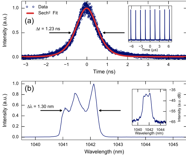
Fig. 3. Characteristics of laser output. (a) Streak camera trace (inset: pulse train on oscilloscope). (b) Optical spectrum on linear scale (inset: log scale).
