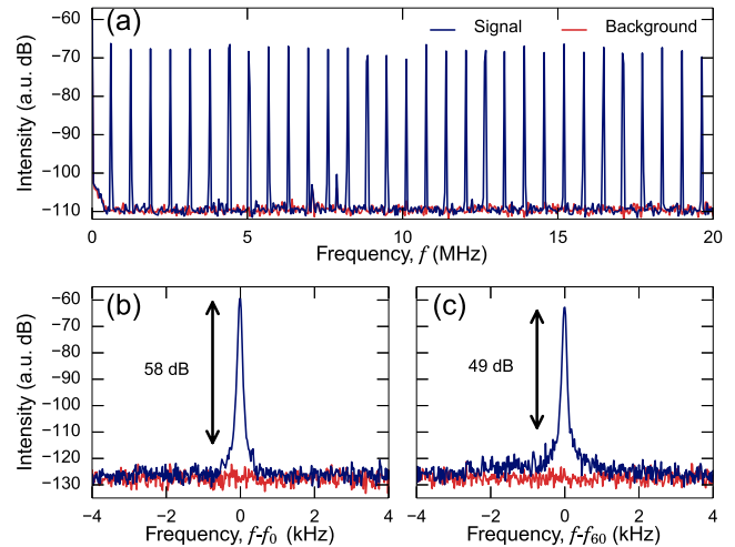
Fig. 4. RF spectrum of laser output: (a) 20 MHz span. (b) 8 kHz span about fundamental frequency, f_0 = 641 kHz. (c) 8 kHz span about 60 th harmonic, f_{60} = 38.46 MHz (30 Hz resolution bandwidth).
