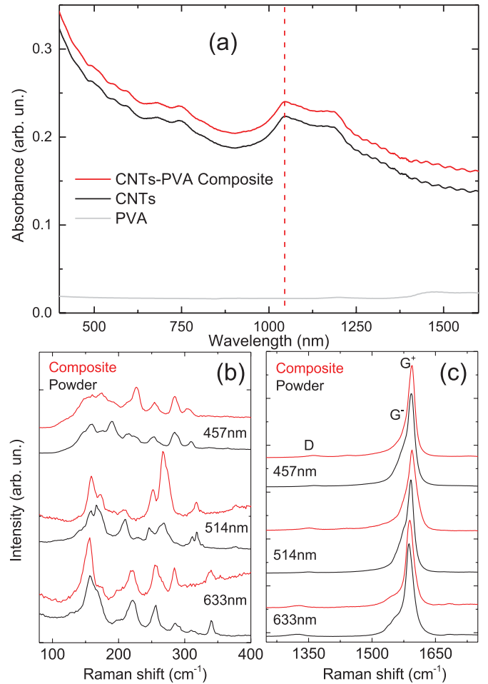
Fig. 1. (a) Absorption spectrum of CNTs (black line), CNT-PVA composite (red line), and PVA (grey line). The operating wavelength is marked by the red dashed line. Raman spectra of CNT powders (black lines) and CNT-PVA composite (red lines) at different excitation wavelengths: (b) RBM region and (c) G region.
