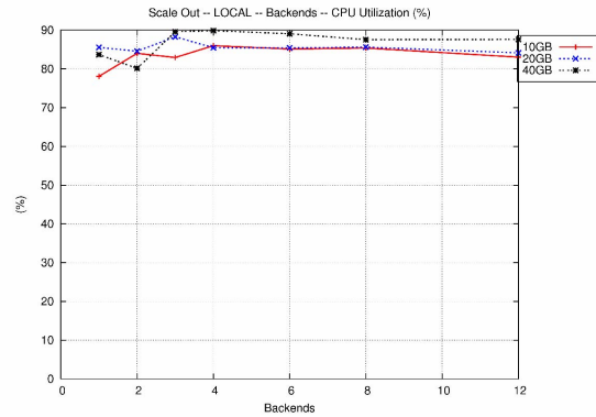
Figure 14: average processor utilization in the back-ends as a function of number of back-ends. Data sets on local disk and ext3 file system.
