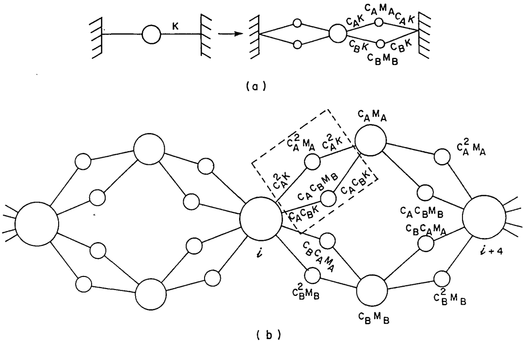
Fig. 5. — Construction of a hierarchical lattice for a mass and spring problem. a ) Each spring of force constant K is replaced by two masses each attached in parallel by two springs whose force constant is as indicated on the figure. In the disordered binary chain problem this lattice can model (see Ref. 13) c_A and c_B are the concentration respectively of the « primitive » masses M_A and M_B ( c_A + c_B = 1 ). \omega^2 in the text is the square of the angular vibration frequency for this problem. b ) Lattice obtained by applying twice the rule described in a ).
