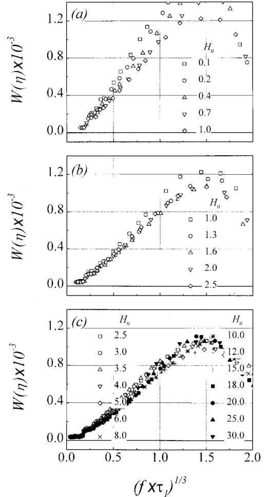
FIG. 8. Power-law dependence of scaling function W on frequency f \times \tau_1 over the low- f range, with an exponent of 1/3 . Here r = -3.0 and u = 1.0 .
