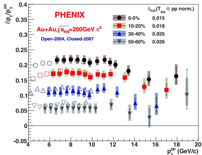
FIG. 3. p_T^{pp} dependence of S_{\text{loss}} for \pi^0 in 200-GeV Au + Au collisions from (solid symbols) 2007 data [8] and (open symbols) 2004 data from the PHENIX experiment at RHIC for p_T < 10 GeV/c [12]. The error boxes corresponding to type- B errors are not shown for year- 2004 data, but the magnitudes are same as the ones for year- 2007 data. \delta_{\text{sys}}(T_{AA} \oplus pp \text{ norm}) are type -C errors and show the absolute amount that the data points would move.
