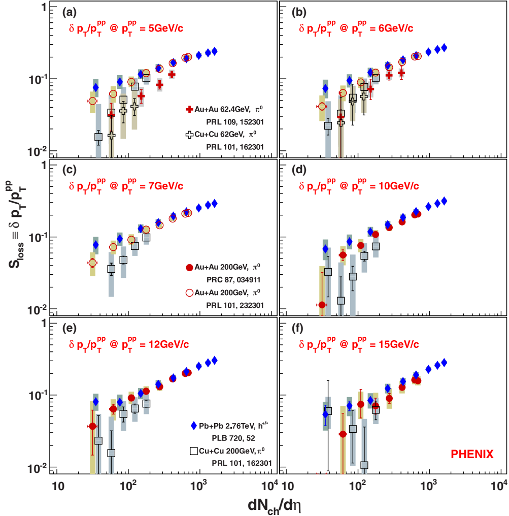
FIG. 14. dN_{\text{ch}}/d\eta dependence of the fractional momentum loss. \delta_{\text{sys}}(T_{AA} \oplus pp \text{ norm}) is not shown in these plots.
