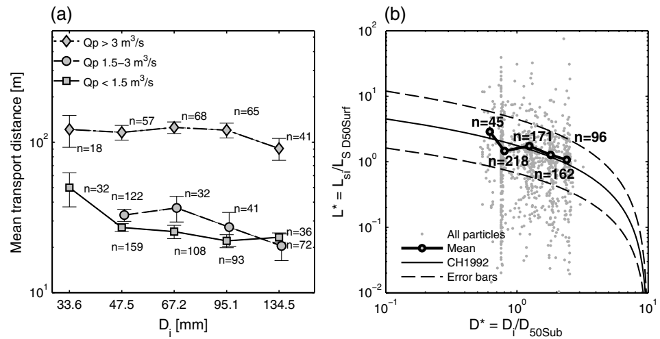
Figure 5. (a) Mean transport distances, with standard errors, for three peak discharge classes ( Q_p < 1.5 \text{ m}^3/\text{s} , 1.5 \leq Q_p < 3 \text{ m}^3/\text{s} , and Q_p \geq 3 \text{ m}^3/\text{s} ), and five particle size classes indexed by their geometric means (33.6–134.5 mm), plotted as a continuous variable on a log scale. (b) Relationship between scaled travel distance ( L^* ) and scaled particle size ( D^* ) for all individual particle movements, and their medians (circles) in five grain-size classes. The transport distance L_{si} of each particle is scaled by the mean displacement of the grain-size fraction containing the D_{50surf} of the streambed surface; D_i is scaled by the D_{50sub} of the subsurface. The thin black line (CH1992) represents Equation (1) with the uncertainty bounds (dashed lines) given by Church and Hassan [1992].
