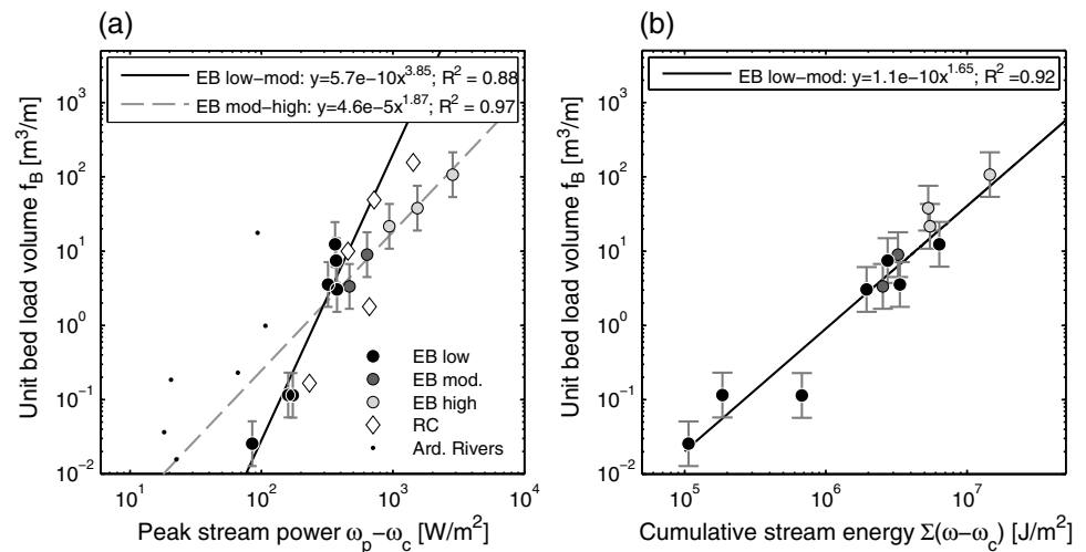
Figure 7. Unit bed load volumes ( f_B ) of the Erlenbach (EB), Rio Cordon (RC) and the Ardennian rivers (Ard. Rivers) related to (a) the excess stream power of the peak discharge and (b) the cumulative excess stream energy over each entire flood event. Black, dark gray and light gray circles indicate survey periods with low, moderate, and high peak discharges ( Q_p ) at the Erlenbach. EB errors for f_B are assumed to be a factor of 2 [Rickenmann and McArdeil, 2008]. Regression lines were derived from the Erlenbach values by functional analysis.
