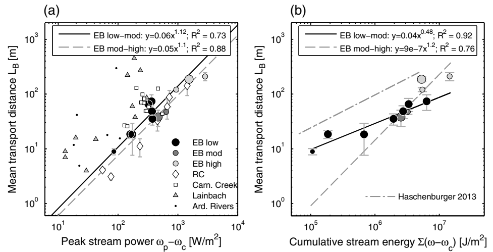
Figure 6. Mean transport distances ( L_B ), related to (a) the excess stream power of the peak discharge and (b) the cumulative excess stream energy over each entire flood event. Black, dark gray, and light gray circles indicate survey periods with low, moderate, and high peak discharges ( Q_p ) at the Erlenbach (EB) (low: Q_p < 1.5 \text{ m}^3/\text{s} ; mod: 1.5 \geq Q_p < 3 \text{ m}^3/\text{s} ; high: Q_p \geq 3 \text{ m}^3/\text{s} ). Small symbols show initial displacements after particle seeding; large symbols show subsequent displacements from “natural” positions for the Erlenbach. Error bars indicate standard errors. The black regression line is derived from functional analysis fitted to the low- to moderate-magnitude events, corrected for log-transformation bias. The dashed gray regression line is fitted to moderate- to high-magnitude events using the same methods. In Figure 6a, mean transport distances at Rio Cordon (RC), Carnation Creek [Haschenburger and Church, 1998], the Lainbach [Gintz et al., 1996] and for several Ardennian Rivers (Ard. Rivers) [Houbrechts et al., 2012] are also shown. In Figure 6b, the relation of Haschenburger [2013] for the Carnation Creek is added.
