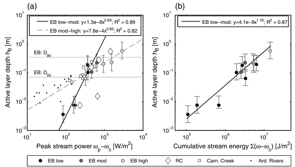
Figure 9. Back-calculated active layer depth related to (a) unit excess stream power of the peak discharge and (b) unit cumulative excess stream energy for the Erlenbach (EB) and Rio Cordon (RC). Black, dark gray, and light gray circles indicate events with low, moderate, and high peak discharges ( Q_p ) at the Erlenbach (EB). The solid black lines were fitted to the Erlenbach low- to moderate-magnitude events ( Q_p < 3 \text{ m}^3/\text{s} ). The dashed black line in Figure 9a was fitted to the moderate- to high-magnitude events ( Q_p \geq 1.5 \text{ m}^3/\text{s} ). Erlenbach error bars are derived from uncertainties in the measured bed load volume (factor 2) and the standard error of the transport distances. Squares represent scour chain measurements in Carnation Creek, Canada [Haschenburger and Church, 1998]. Small black dots (Ard. Rivers) are based on scour chain measurements in several Ardennian Rivers, Belgium [Houbrechts et al., 2012]. The black and dashed gray lines were not fitted to data from Rio Cordon, Carnation Creek, or the Ardennian Rivers.
