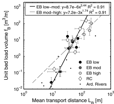
Figure 8. Unit bed load volumes ( f_B ) as a function of mean transport distance ( L_B ) for the Erlenbach (EB), Rio Cordon (RC), and the Ardennian rivers (Ard. Rivers). Black, dark gray, and light gray circles indicate events with low, moderate, and high magnitude peak discharges ( Q_p ) at EB. EB errors for f_B are assumed to be a factor of 2 [Rickenmann and McArdell, 2008] and error bars for L_B show the standard error of the transport distances. The black regression line is fitted to the EB low- to moderate-magnitude events, and the dashed gray regression line is fitted to the moderate- to high-magnitude events.
