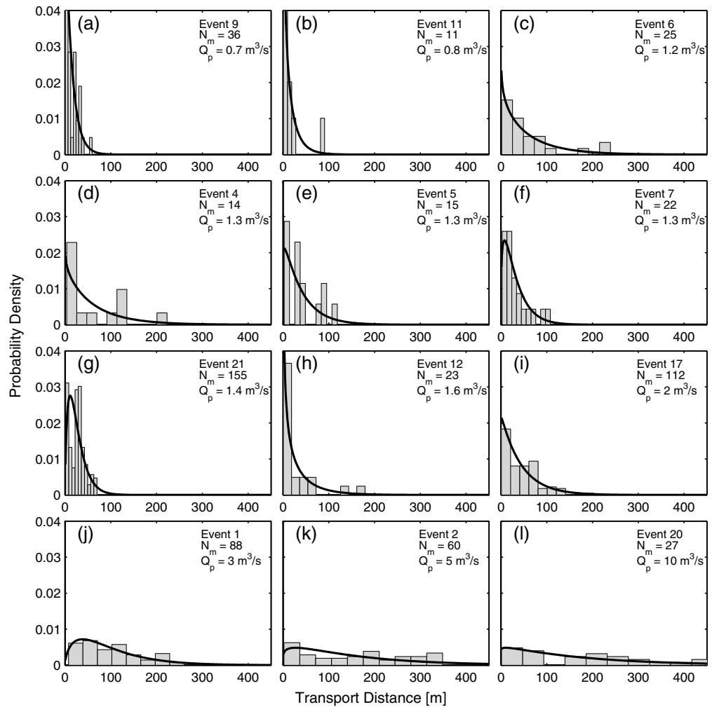
Figure 4. Tracer transport distance histograms for selected transport events sorted (a–l) according to peak discharge ( Q_p ), with fitted gamma distributions (heavy black lines). N_m is the number of moved tracers that the histograms are based on.
