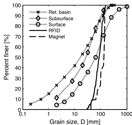
Figure 2. Grain-size distributions of the sediment deposited in the Erlenbach retention basin (crosses), of the channel bed subsurface and surface (diamonds and circles, respectively), and of the RFID and magnetic tracer populations (solid and dotted lines, respectively).
