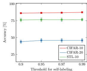
Fig. 6: Ablation threshold during self-labeling step.
