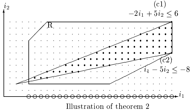
Illustration of theorem 2
