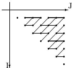
Figure 13: Tiling H^T_3
