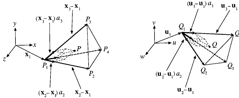
Fig. 4 Tetrahedron P_1P_2P_3P_4 in the x,y,z space is mapped by the 3D transformation f:\mathbb{R}^3\rightarrow\mathbb{R}^3 into tetrahedron Q_1Q_2Q_3Q_4 in the u,v,w space. The point P is mapped by linear tetrahedral interpolation into the destination point Q . The coordinates of points P_1, P_2, P_3, P_4 , and P are \mathbf{x}_1=(x_1,y_1,z_1), \mathbf{x}_2=(x_2,y_2,z_2), \mathbf{x}_3=(x_3,y_3,z_3), \mathbf{x}_4=(x_4,y_4,z_4) , and \mathbf{x}=(x,y,z) , and the coordinates of points Q_1, Q_2, Q_3, Q_4 , and Q are \mathbf{u}_1=(u_1,v_1,w_1), \mathbf{u}_2=(u_2,v_2,w_2), \mathbf{u}_3=(u_3,v_3,w_3), \mathbf{u}_4=(u_4,v_4,w_4) , and \mathbf{u}=(u,v,w) .
