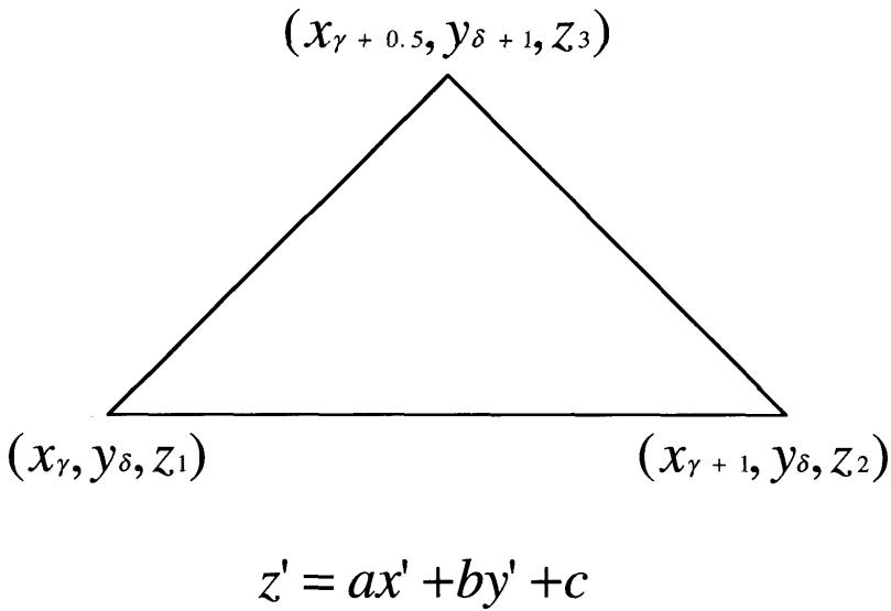
Figure 5. Definition of surface plane through triangle.
