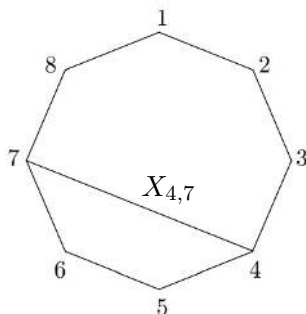
Figure 15. The diagonal (4,7) subdivides the 8-gon into a 4-gon (on the “left”) and a 6-gon (on the “right”), suggesting that the facet X_{4,7} = 0 of the associahedron \mathcal{A}_{n=8} is combinatorially identical to \mathcal{A}_{n=4} \times \mathcal{A}_{n=6} .
