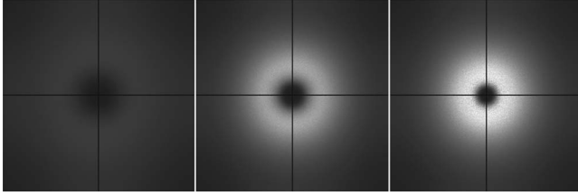
FIG. 4. Experimentally determined image structure function D(\mathbf{q}, \Delta t) for the images \Delta I(\mathbf{x}; \Delta t) in Fig. 2: \Delta t=0.01 s, \Delta t=0.1 s, and \Delta t=1 s. Each image is the result of an average over 2000 statistically independent \Delta I images with the same \Delta t . The black cross at the center of each image is the result of a postprocessing operation and is used to suppress artificially large contributions due to image processing artifacts. The larger energy content of the right image can be appreciated.
