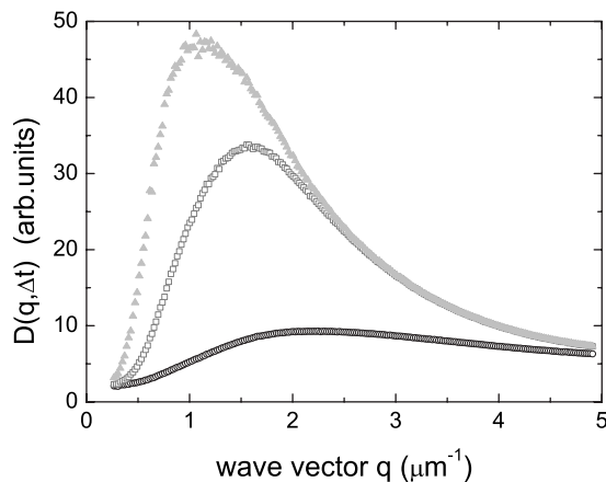
FIG. 5. The image structure function D(q, \Delta t) is plotted as a function of q for different values of \Delta t : \Delta t=0.01 s (open circles, black), \Delta t=0.1 s (open squares, dark gray), and \Delta t=1 s (close up triangles, light gray).
