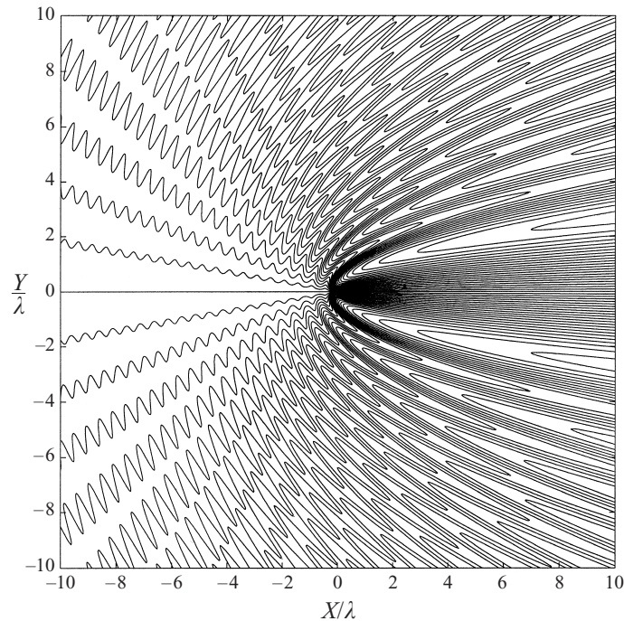
FIGURE 2. Contour plot of P_{21}^{\text{rms}}/(\Gamma \omega/2\pi) as a function of X/\lambda , where \lambda = 2\pi/k is the wavelength of the incident wave. Contour interval: 0.25. Note that P_{21}^{\text{rms}} vanishes on the X -axis.
