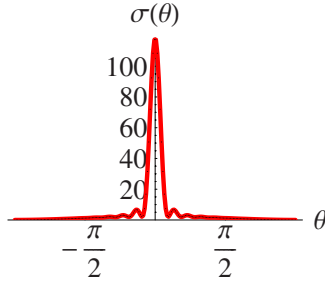
FIG. 5. (Color online) Angular dependence of the cross section when the cluster is determined by a mass term, which breaks the symmetry between the sublattices. The parameters used are kFR = 10 and \Delta R/v_F = 20 .
