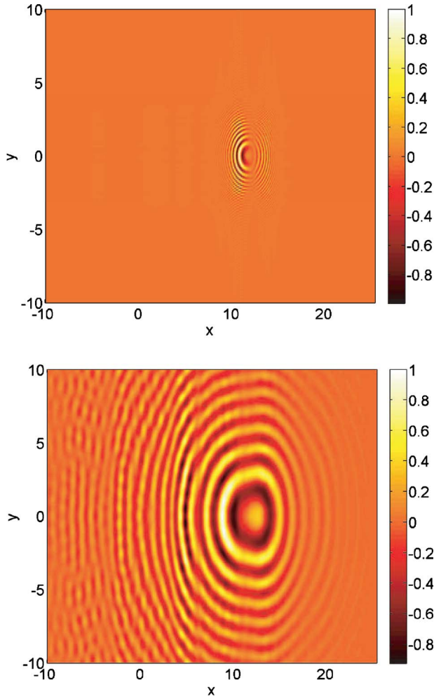
Fig. 5. (Color online) Contour plots of the image I(x, y) defined in Eq. (5.5) corresponding to a single point obstacle shown in Fig. 4 for the Dirichlet (top) and Neumann (bottom) cases.
