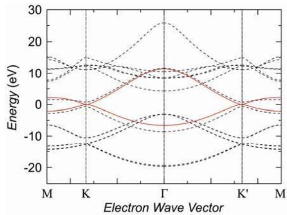
FIG. 9 (color online). Ab initio electron band structure of graphite. The red lines indicate the \pi and \pi^* bands, i.e. valence and conduction bands, respectively, along \Gamma -K-M direction used in the electron scattering analysis. Dashed lines indicate \sigma and \sigma^* bands.
