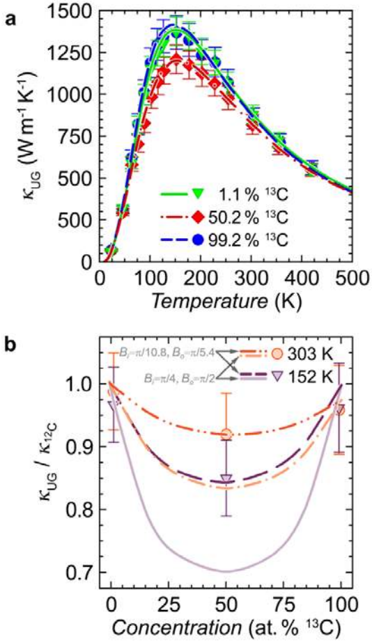
FIG. 4 (color online). (a) Solid thermal conductivity of the UG ( \kappa_{UG} ) versus temperature for 13 C concentration of 1.1% (green down triangles), 50.2% (red diamonds), and 99.2% (blue circles). The lines are the calculated thermal conductivity based on the fitting parameters discussed in the text for different 13 C concentrations. (b) Calculated solid thermal conductivity normalized by the theoretical value for isotopically pure 12 C graphite ( \kappa_{UG}/\kappa_{12C} ) as a function of 13 C isotopic concentration at temperatures of 152 K (purple down triangles) and 303 K (orange circles). In one calculation, the isotope scattering coefficient B is taken to be B_i = \pi/4 for the in-plane mode and B_o = \pi/2 for the out-of-plane modes. In another calculation, the two B coefficients are reduced to B_i = \pi/10.8 for the in-plane mode and B_o = \pi/5.4 .
