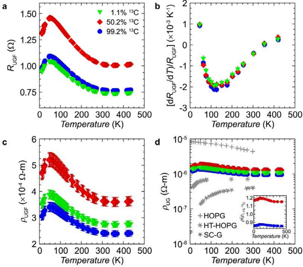
FIG. 2 (color online). Temperature-dependent electrical properties of ultrathin graphite foam (UGF) after post-synthesis annealing. The isotopic concentration of ^{13}\text{C} in ^{12}\text{C} for the UGF samples is 1.1% (green down triangles), 50.2% (red diamonds), and 99.2% (blue circles). (a) Measured low-bias electrical resistance ( R_{\text{UGF}} ) and (b) normalized low-bias resistance change with temperature at each temperature [(dR_{\text{UGF}}(T)/dT)/R_{\text{UGF}}(T)] . (c) Electrical resistivity ( \rho_{\text{UGF}} ) of the UGF. (d) Solid electrical resistivity of the ultrathin graphite ( \rho_{\text{UG}} ) within the UGF, calculated using the foam theory of Lemlich [27], \rho_{\text{UG}} = (\phi/3)\rho_{\text{UGF}} , where \phi is the volume fraction. Shown in comparison are values for highly oriented pyrolytic graphite deposited at 2250°C (HOPG, gray crosses) [57], HOPG deposited at 2200°C and subsequently heat treated at 3200°C (HT-HOPG, gray asterisks) [10], and single crystal graphite (SC-G, gray stars) [58]. (d, inset) \rho_{\text{UG}} of the 50.2 and 99.2 at.% ^{13}\text{C} samples normalized by that of the 1.1 at.% ^{13}\text{C} sample. The legend shown in panel (a) applies to panels (a–d).
