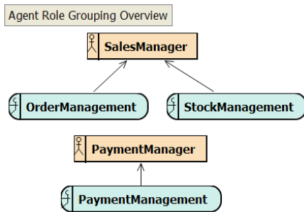
Figure 9: Agent-Role Diagram
