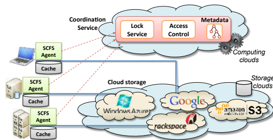
Figure 2: SCFS architecture with its three main components.
