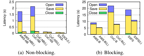
Figure 8: Latency of a personal storage service actions (see Figure 7) in a file of 1.2MB. The (L) variants maintain lock files in the local file system. All labels starting with CoC or AWS represent SCFS variants.
