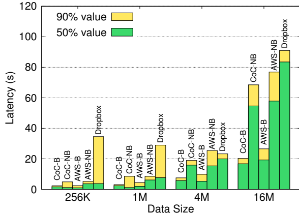
Figure 9: Sharing file 50th and 90th latency for SCFS (CoC B and NB, AWS B and NB) and Dropbox for different file sizes.
