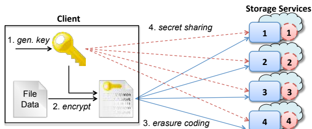
Figure 6: A write in SCFS using the DepSky protocols.
