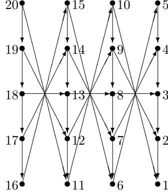
Figure 3: The dependence graph for SARE S . The numbers indicate a serial schedule.
