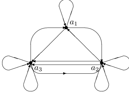
Figure 1: The RDG for the system of recurrence equations of Ex. 1.
