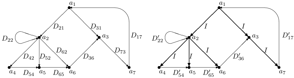
Figure 2: The RDG before (on the left) and after (on the right) the tree conversion.
