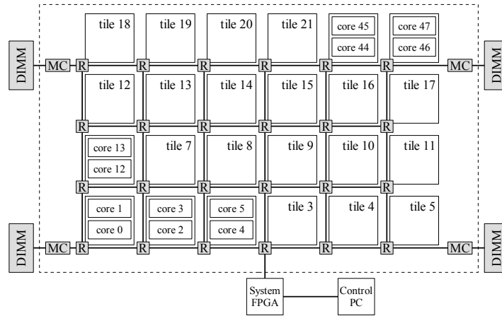
Fig. 1. Intel SCC block diagram
