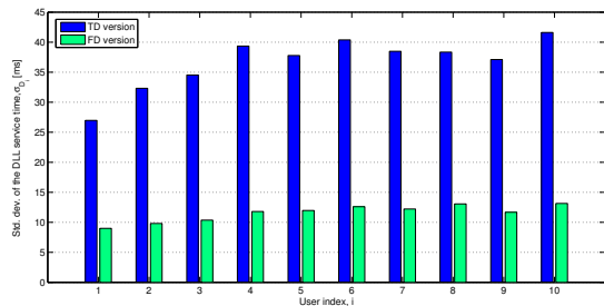
Fig. 10. \sigma_{D_i} for the TD and FD approach, over a time dispersive channel with Doppler spread \nu_d = 120 Hz.
