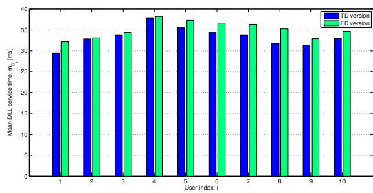
Fig. 9. Mean DLL service time m_{D_i} for the TD and FD approach, over a time dispersive channel with Doppler spread \nu_d = 120 Hz.
