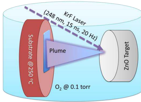
Figure Appx. I. 1. A schematic diagram of the alignment in PLD chamber.
