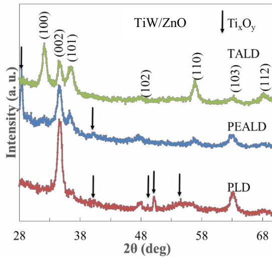
Figure Appx. I. 4. GAXRD profiles of ZnO thin film synthesized by TALD at 200 °C, PEALD at 200°C and PLD at 250°C. Titanium oxide (Ti x O y ) phases were detected in both PLD-ZnO and PEALD-ZnO.
