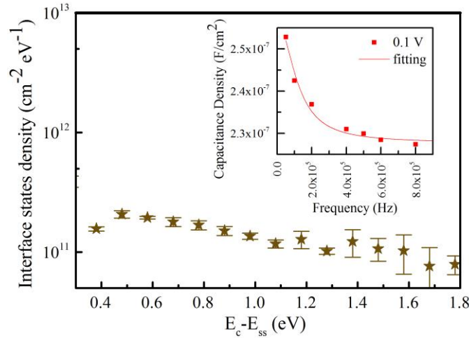
Figure 5.22. Energy distribution curve of the interface states fitted from C_p - f data for P-50-Pt. ( Inset: The C_p - f characteristics of the Schottky diode at 0.1 V forward bias. The solid line presents the functional fitting)
