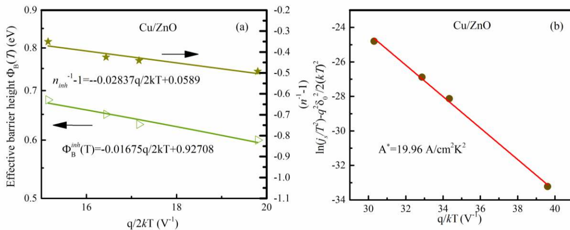
Figure 5.32 The \Phi_B(T) versus q/2kT and (n^{-1} - 1) versus q/2kT plots with linear approximation for Cu/ZnO diode; (b) modified Richardson plot of \ln(j_s/T^2) - q^2 \delta_0^2 / 2(kT)^2 versus q/kT for Cu/ZnO diode.
