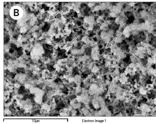
Fig. 6. Scanning electron photomicrograph of Millipore® membrane(A) and Ca-P coated Millipore® membrane(B). Arrows indicate 0.45µm sized pore and there was no change in pore size after Ca-P coating. (SEM, ×5000)
