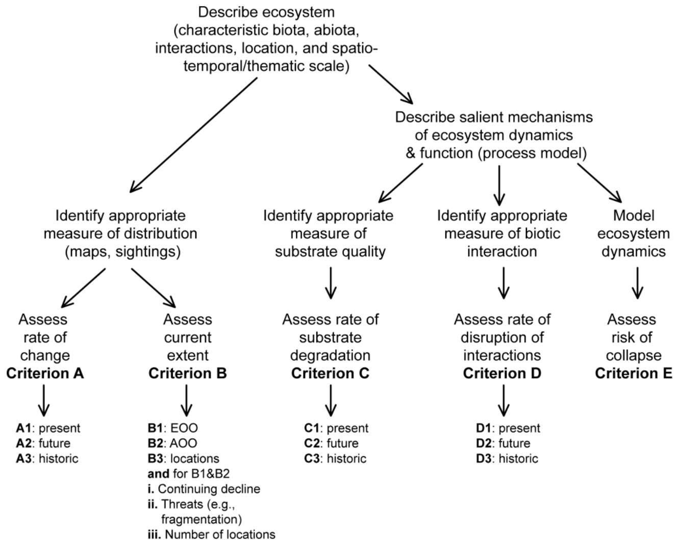
Figure 3. Protocol for assessing the risk of collapse of an ecosystem using proposed Red List criteria v2.0 (see Table 3). doi:10.1371/journal.pone.0062111.g003
