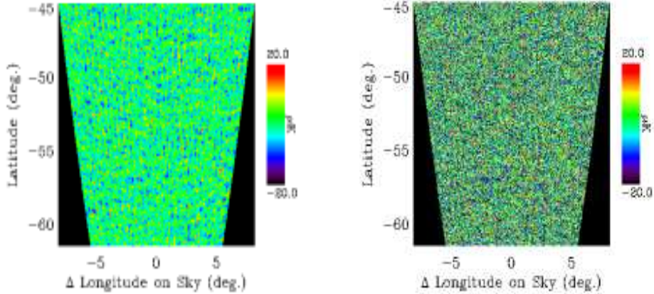
Figure 6. Simulated polarization maps from QUaD (left) and Planck (right), showing a 300 \text{ deg}^2 field of Q-mode anisotropies at 150 GHz. All of the structure in the high signal-to-noise QUaD map is real signal, while the Planck map (shown with the same pixelization) has much lower signal-to-noise per pixel. Foregrounds and other systematic effects are not included in either map.
