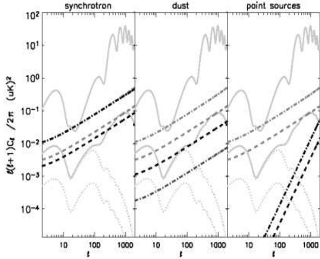
Figure 2. Models used for vibrating dust, synchrotron emission and residual point sources (black) compared to the EE and BB power spectra (light grey, solid). The different lines show foreground models at 100 GHz (dash-dot) and 150 GHz (dash). The total foreground power spectra are also shown on each plot (dark grey). The GW component of the BB-spectra is shown for r = 0.1 (upper dotted line) and r = 0.01 (lower dotted line). The other foregrounds are either unpolarized or can be neglected
