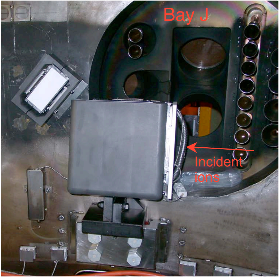
Figure 5: Photograph of the sFLIP inside the NSTX vacuum vessel.
