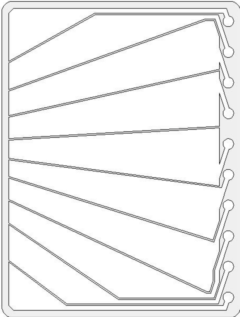
Figure 6: Drawing of the Faraday cup strip pattern on the phosphor substrate. The plate is 15.0 x 20.0 cm and the apertures lie at the edge of the plate where the tapered strips converge. The strips are numbered 1 to 10 running from top to bottom in this image, extending from lowest to highest pitch angles, correspondingly.
