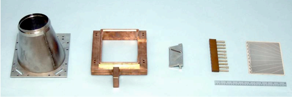
Figure 3: Exploded view of the sFLIP in-vessel components, showing (left to right) the conical light shield, copper frame, aperture block, Faraday cup spring contact assembly, and the scintillator plate. A 30 cm ruler is show below the scintillator plate for scale.
