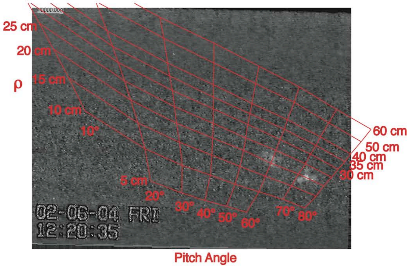
Figure 7: Fast ion loss image from NSTX shot 111192 at 253 ms. The image is overlaid with a grid in pitch angle and gyroradius centroid for interpretation. Note the two luminous spots registered toward the right edge of the image. These arise from neutral beam ions being lost at two different pitch angles and then striking the scintillator.
