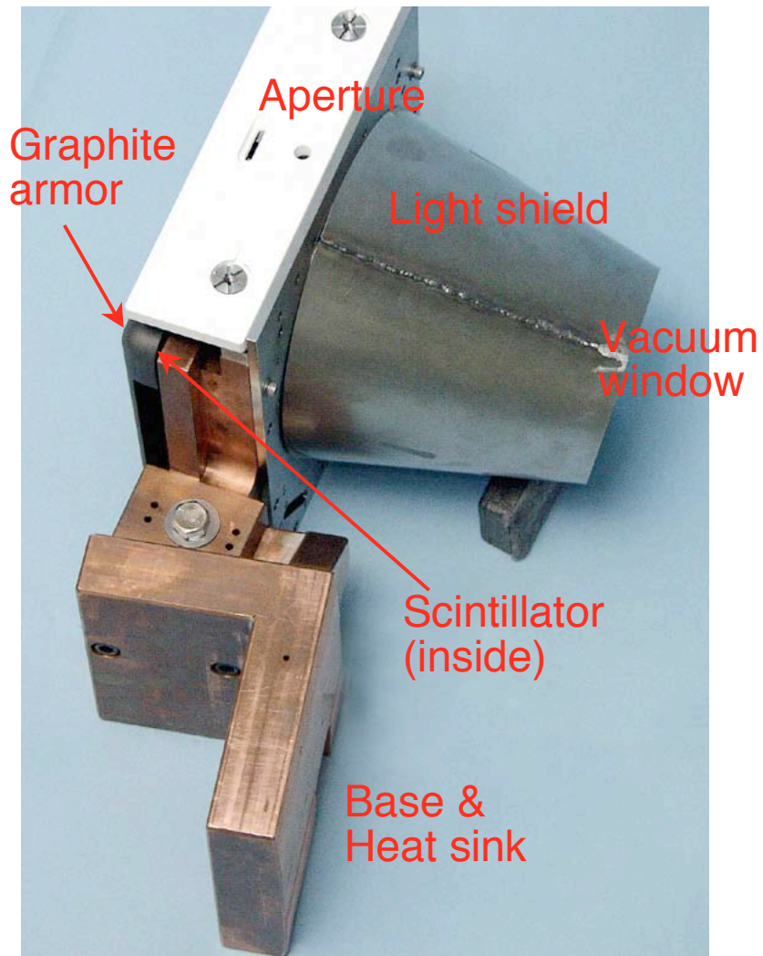
Figure 4: Photograph of the sFLIP assembly
