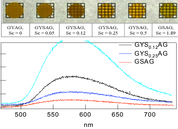
Fig. 8. Beta-excited radioluminescence spectra of Cerium doped Gadolinium-based garnet ceramics. Spectra have been corrected for sensitivity.
