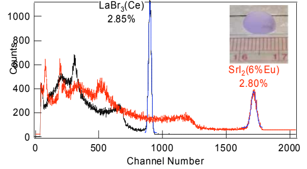
Fig. 4. Energy resolution of the Strontium Iodide crystal shown in the photo inset, reveals comparable energy resolution to that of \text{LaBr}_3(\text{Ce}) .
