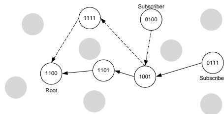
Fig. 4. Base Mechanism for Subscription and Multicast Tree Creation.
