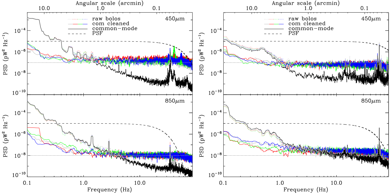
Figure 2. Bolometer power spectral densities (PSDs) for the same two data sets (before and after upgrades) used in Fig. 1. The PSDs have been boxcar smoothed with a width of 0.1 Hz to reduce the noise slightly and clarify some features. Four of the most sensitive bolometers have been selected at each wavelength, and the flat-fielded and step-corrected (but otherwise raw) PSDs are shown as coloured dotted lines (the blue signals are for the same time series as those shown in Fig. 1). The solid black lines are the PSDs of the common-mode signals at each wavelength, and the solid coloured lines show the PSDs of the bolometers once the common-mode is removed. Finally, the dashed black lines show the spectral shape produced by a point source given the scan speeds for the two observations ( 120 \text{ arcsec s}^{-1} in (a), and 190 \text{ arcsec s}^{-1} in (b)); for reference, the top horizontal axes shows the conversion from frequency to angular scale. Horizontal dotted lines at 10^{-7} and 10^{-8} \text{ pW Hz}^{-1} at 450 and 850 \mu\text{m} , respectively, are provided as a visual reference for the white-noise levels. In addition to 1/f and white noise components, and line features, all of the PSDs exhibit the gradual roll-off of the anti-aliasing filter just below the Nyquist frequency. (a) For the S2SRO data, particularly at 450 \mu\text{m} , there are broad line features in the PSDs at both wavelengths above \sim 35 \text{ Hz} . At lower frequencies, the bolometer signals exhibit clear 1/f knees at approximately 2 and 3 Hz at 450 and 850 \mu\text{m} . Common-mode subtraction removes most of the correlated fringe oscillation signal, lowering the 1/f knees to approximately 0.6 and 1.0 Hz at 450 and 850 \mu\text{m} , respectively. (b) Data from the fully-commissioned instrument tend to have lower 1/f knees, and fewer line features. For this example, the improvement is most striking at 450 \mu\text{m} where the PSD is approximately two orders-of-magnitude lower in the fully-commissioned data at 0.1 Hz. The white noise performance, however, is similar for the two subarrays (s4a and s8b) that were used both before and after the upgrades.
