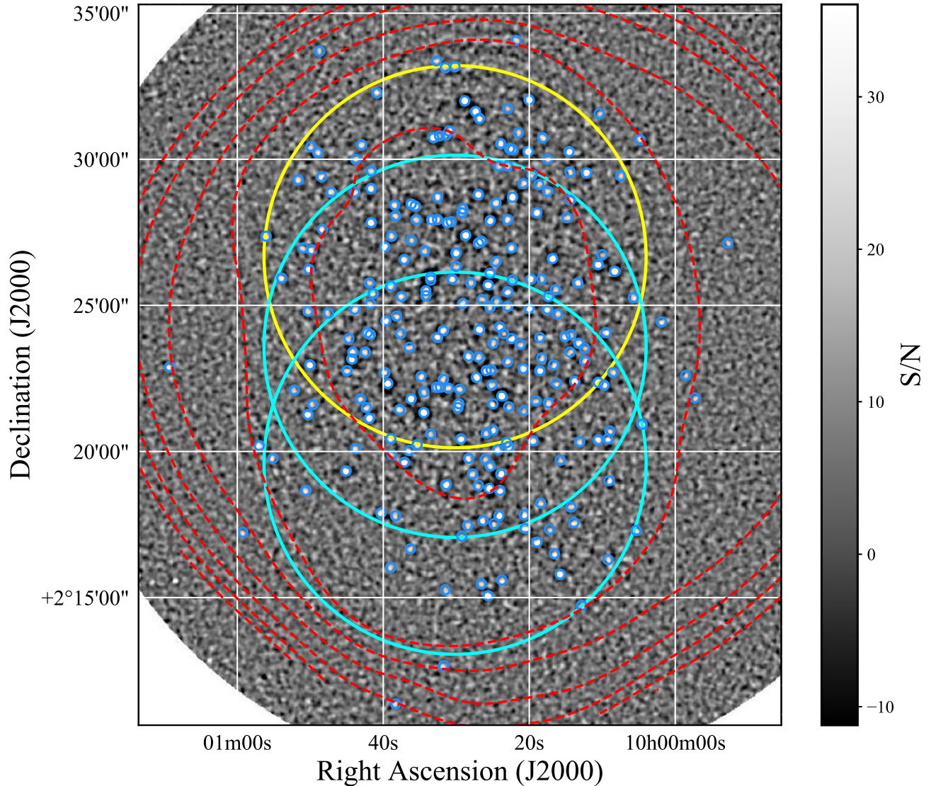
Figure 1. The JCMT SCUBA-2 450\text{-}\mu\text{m} S/N image, with the positions of the 256 S/N > 4 sources (blue circles). The large yellow and cyan circles indicate the deep scan regions of STUDIES and S2CLS, respectively. The deep area of C13 covers the entire area of this image. The overlapping region is the deepest area ever observed in the 450\text{-}\mu\text{m} waveband. The red dashed contours show the instrumental noise, with contour levels of 1, 4, 7, 10, 13, 16, and 19 mJy.
