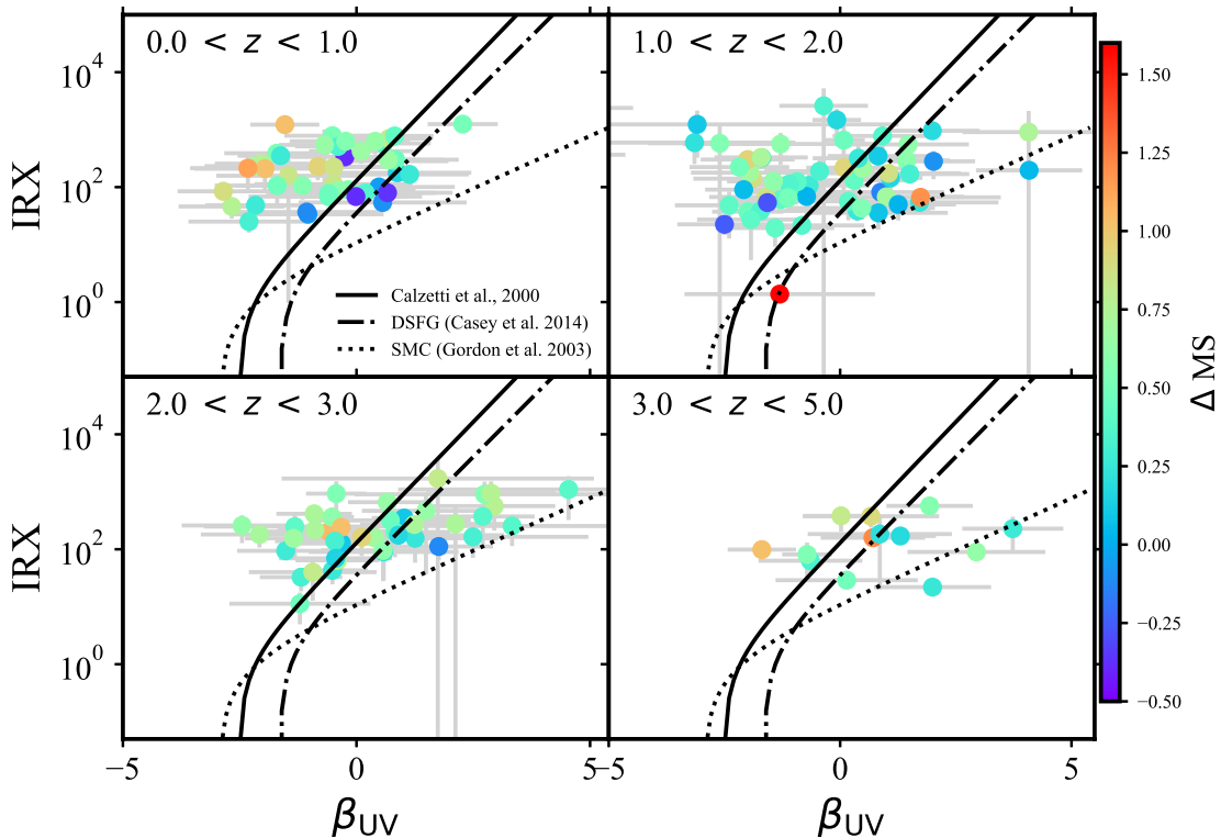
Figure 15. The infrared excess (IRX) versus ultra-violet slope ( \beta_{UV} ), color-coded by \Delta MS . Our sample shows no obvious correlation in the IRX- \beta_{UV} plane. For comparison, we plot attenuation curves from the SMC (dotted lines; Gordon et al. 2003), local starburst galaxies (solid lines; Calzetti et al. 2000), and local ( z < 0.085 ) DSFGs (dotted-dashed lines, Casey et al. 2014b).
