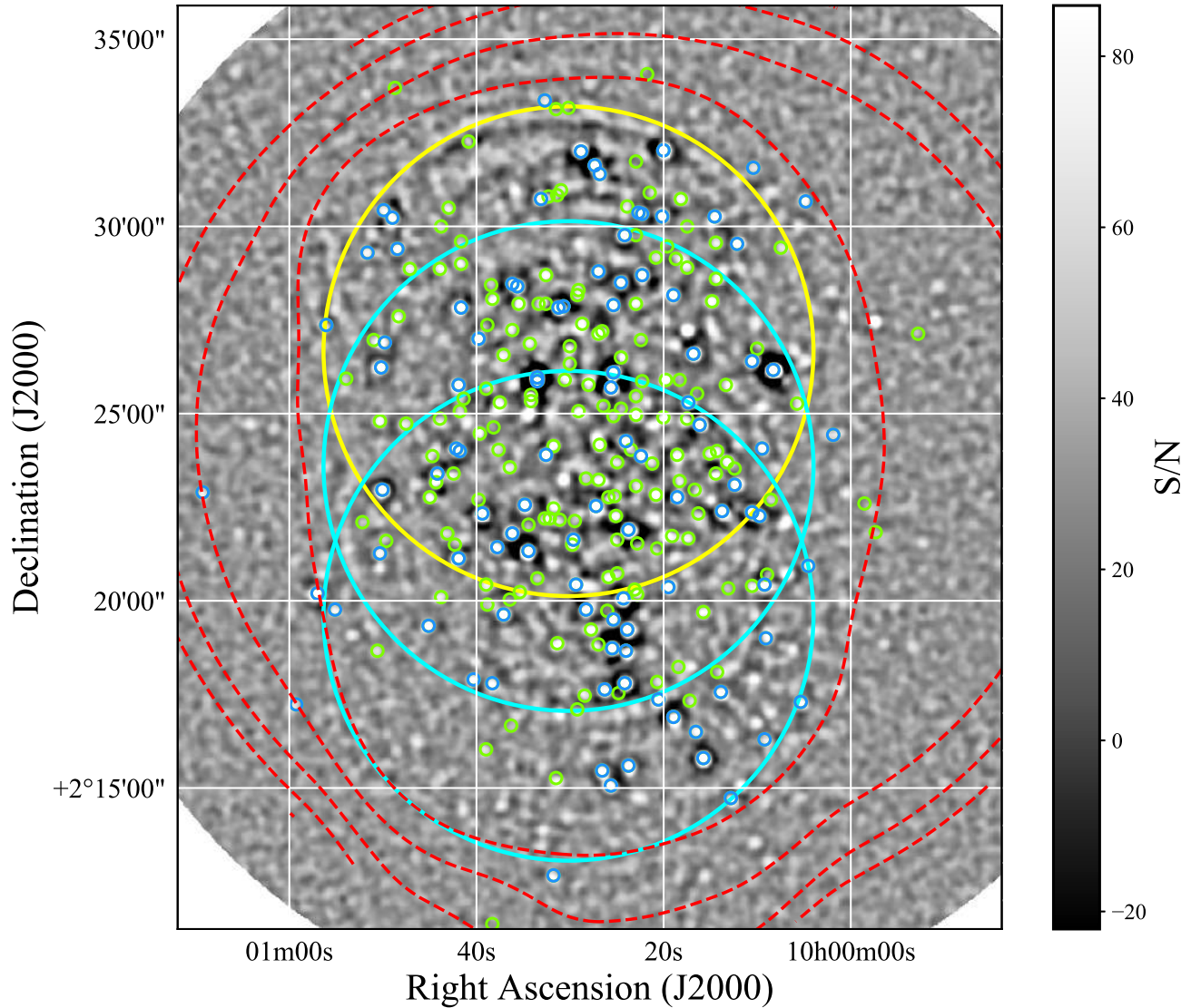
Figure 2. The JCMT SCUBA-2 850- \mu\text{m} S/N image. All 450 \mu\text{m} detected sources are circled on this map, while the 157 sources without high-significance 850- \mu\text{m} flux densities ( < 2.1 mJy) are shown in green. The high values of S/N will decrease by a factor of roughly 3 when taking into account confusion noise ( \sigma_c = 0.42 mJy; see Appendix B). The red dashed contours show the instrumental noise with contour levels of 0.7, 1.4, 2.1, and 2.8 mJy. The meaning of the large yellow and cyan circles is the same as in Figure 1.
