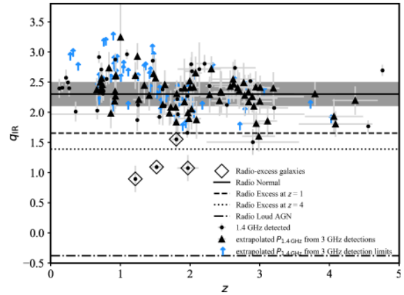
Figure 9. Shown is q_{\text{IR}} vs. z for our 450- \mu\text{m} sample. Our sample follows the tight local FIR–Radio correlation (solid line; Condon 1992), while the shaded area represents the \pm 1\sigma dispersion in the local correlation. The four sources enclosed by diamonds are classified as radio-excess galaxies, although none of them exceed the threshold for radio-loud AGNs (see §4.1). The lower limits of q_{\text{IR}} for those sources without 3-GHz detections are shown as upward-pointing arrows. Their S_{1.4\text{ GHz}} are extrapolated from the 5\sigma detection limit of S_{3\text{ GHz}} = 13\ \mu\text{Jy} by assuming our typical \alpha_r .
