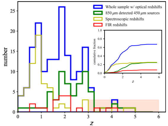
Figure 6. Redshift distribution of our sample with optical redshifts (blue histogram) and 850- \mu\text{m} detections (green histogram). The medians of these two distributions are z = 1.79^{+0.03}_{-0.15} and z = 2.30^{+0.27}_{-0.26} , respectively. The vast majority of our sample lies at z \lesssim 3 . The distribution of the 65 galaxies with spectroscopic redshifts is shown with the yellow histogram, which is clearly biased toward low redshifts. The distribution of the 19 sources with z_{\text{FIR}} is shown with the red histogram. A significant fraction (46/256) of our sources do not have redshift determinations, since they do not have 24- \mu\text{m} or radio identifications and consequently lack optical counterparts. If they are at z > 3 (see §3.3) and have a flat redshift distribution between z = 3 and 6, they are represented by the orange shaded area in this diagram. The small panel shows the cumulative redshift completeness in each sub-sample among the 256 4\sigma sources.
