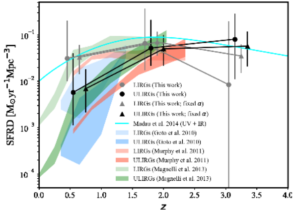
Figure 20. SFRD versus redshift, breaking down by LIRG and ULIRG contributions. Our estimations are shown as gray points (LIRGs) and black points (ULIRGs). The horizontal displacement between the two measurements is artificial, to avoid confusion. The results from Magnelli et al. 2013, Goto et al. 2010, and Murphy et al. 2011 are shown as green, blue, and red shaded regions ( 1\sigma scatter), respectively. The cyan curve shows the total SFRD from Madau & Dickinson (2014).
