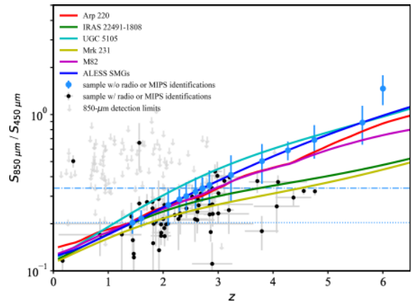
Figure 4. Flux density ratio of 850–450 \mu\text{m} versus redshift. The colored curves represent the flux density ratios derived from various SED templates: Arp 220* (ULIRG), IRAS 22491-1808* (ULIRG), UGC 5105* (ULIRG with AGN), Mrk 231* (ULIRG with AGN), M82* (luminous starburst galaxies), and averaged SED from ALESS (da Cunha et al. 2015). For the 15 sources that do not have any radio or 24- \mu\text{m} counterparts but do have 850- \mu\text{m} detections; we place them along the averaged ALESS SED track up to z \simeq 6 , according to their observed flux ratios. The median of the flux density ratio is 0.34^{+0.07}_{-0.02} (blue dotted-dashed line), indicating that they may be SMGs at z \gtrsim 3 . The smallest flux ratio is 0.20 \pm 0.03 (blue dotted line), still placing the SMG at z \gtrsim 1.5 . We also show the S_{850 \mu\text{m}}/S_{450 \mu\text{m}} flux density ratios of our identified sources (black points) that have redshift determinates (§4.2) and the upper limits considering an 850- \mu\text{m} flux threshold given by 2.1 mJy (confusion limit) from the rest of the sample. Our sample is in broad agreement with most of the SED tracks. *Spectral templates of nearby infrared-luminous galaxies are from the Spectral Atlas of Infrared Luminous Galaxies ( http://www.stsci.edu/hst/observatory/crds/non-stellar.html ).
