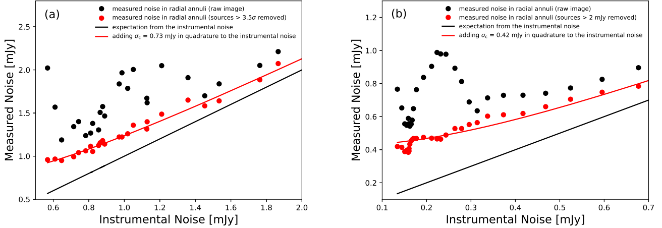
Figure B.2. (a) Measured 450 \mu\text{m} noise in radial annuli as a function of the mean instrumental noise in each annulus. The black points show the noise measured from the raw image, while the red points represent the flux dispersion measured in the image after the sources that are > 3.5\sigma are removed. The black curve shows the mean instrumental noise, and the red curve shows the result when \sigma_c = 0.73 mJy is added in quadrature to the instrumental noise. (b) Same as panel (a) but for 850 \mu\text{m} . The red points show the flux dispersion measured in the image after the sources brighter than 2 mJy are removed. The red curve shows the result when \sigma_c = 0.42 mJy is added in quadrature to the instrumental noise.
