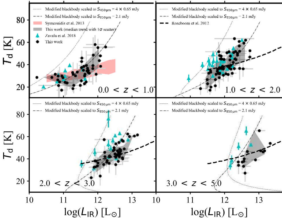
Figure 12. T_d versus L_{\text{IR}} for our 450- \mu\text{m} sample (black circles) and other populations. The dark shaded areas show the running medians of our sample and the 1\sigma scatters. The red shaded area shows the range of 1\sigma scatter of the z = 0 – 1 Herschel /SPIRE-selected LIRGs/ULIRGs from Symeonidis et al. (2013). The dashed curves are the relation derived from z > 1.5 Herschel /SPIRE-selected sources in Roseboom et al. (2012). The triangles are 450- \mu\text{m} -selected SMGs from the shallower SCUBA-2 survey of Zavala et al. (2018). To demonstrate the effects of selection, we convert our flux detection limits to the L_{\text{IR}} sensitivity limits at a given T_d using a modified blackbody under detection limits corresponding to a 450- \mu\text{m} noise of 0.65 mJy (dotted curves) and the 850- \mu\text{m} confusion limit of 2.1 mJy (dash-dotted curves) in the middle of the redshift bins.
