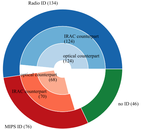
Figure 3. Doughnut chart showing the breakdown of 450\text{-}\mu\text{m} sources into different classes of counterpart identifications. The outer ring shows the number of 450\text{-}\mu\text{m} sources identified at VLA 3 GHz and MIPS 24\text{ }\mu\text{m} , and the unidentified sources, while the middle ring shows the number of IRAC counterparts, which are identified based on their corresponding radio or MIPS positions. Most of these IRAC counterparts have optical counterparts in the COSMOS2015 catalog (inner ring).
