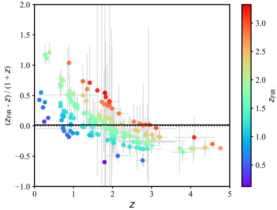
Figure 5. Comparisons of the FIR-derived redshifts ( z_{\text{FIR}} ) with the optical redshifts ( z ), color-coded with z_{\text{FIR}} . The z_{\text{FIR}} estimates are consistent with the optical redshifts with a median offset of 0.01^{+0.02}_{-0.03} (solid horizontal line). The trend of z_{\text{FIR}} being systematically higher than the optical redshift at z < 2 and lower at z > 2 is probably caused by our single-temperature assumption of the SED template and/or the effect of the luminosity– T_{\text{d}} correlation (§5.2), plus selection effects.
