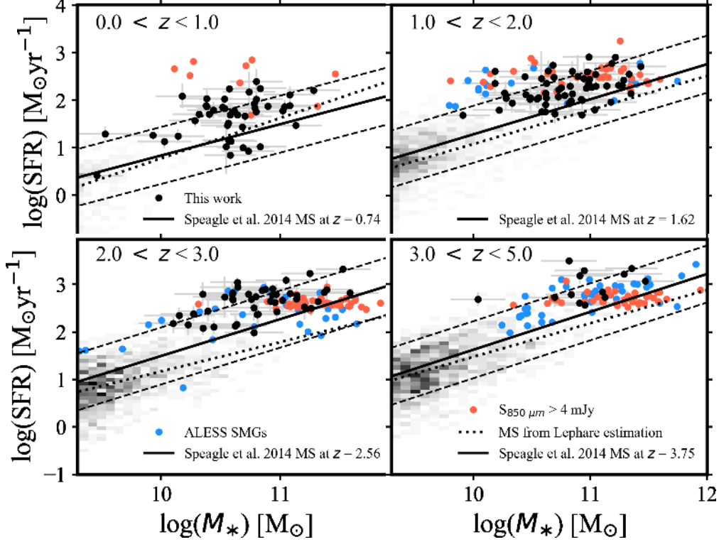
Figure 10. The SFRs as a function of stellar mass for our sample. The gray scales and dotted lines represent the distributions and relations from normal star-forming galaxies in the COSMOS2015 catalog, respectively. The redshift-dependent relations from Speagle et al. (2014) are shown with solid lines, while their \pm 0.6 dex ranges are shown with dashed lines. A sample of bright SCUBA-2 SMGs ( S_{850\ \mu\text{m}} > 4\ \text{mJy} ; Michałowski et al. 2017) is shown with red points, and ALESS SMGs (da Cunha et al. 2015) are shown with blue points.
