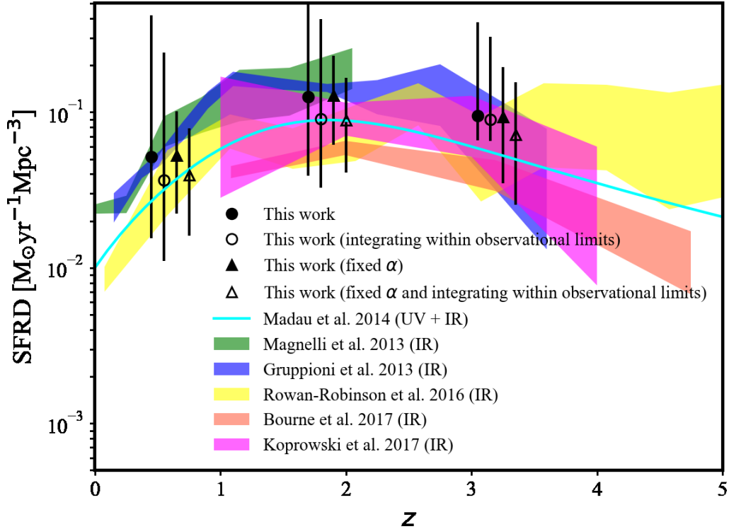
Figure 19. SFRD versus redshift. Our estimations are shown as black filled (integrated from 0.03 L_* to 10^{13.5} L_\odot ) and open (integrated from the minimum observational limits to 10^{13.5} L_\odot ) symbols. The circles and triangles show the results from the cases of free and fixed \alpha , respectively. The horizontal displacements between the symbols are artificial, to avoid confusion. For comparison, we also show the Herschel -based studies (Gruppioni et al. 2013; Magnelli et al. 2013; Rowan-Robinson et al. 2016), as well as SCUBA-2-based studies (Bourne et al. 2017; Koprowski et al. 2017). The width of the shaded areas represents the range of \pm 1\sigma scatter of the corresponding data sets. The solid cyan curve shows the best-fit evolution function of SFRD from Madau & Dickinson (2014) using rest-frame far-ultraviolet or mid-to-FIR data from a variety of galaxy surveys.
