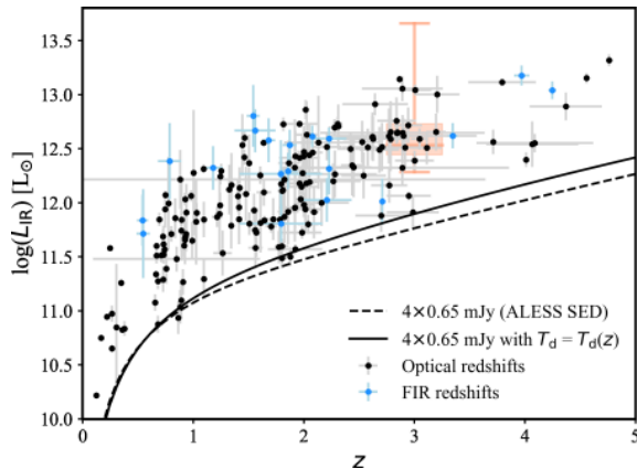
Figure 8. The L_{\text{IR}} as a function of redshift. Our samples that have optical redshifts are shown as black points, while the 19 sources that have z_{\text{FIR}} estimates are shown as blue points. The orange box shows the infrared luminosity range of \log(L_{\text{IR}})=12.3\text{--}13.7 L_{\odot} for the 46 sources without 24- \mu\text{m} or radio identifications, if we place them at their plausible median redshift of z = 3 (see §3.3) and scale their 450- \mu\text{m} flux densities to L_{\text{IR}} using the averaged ALESS SMG SED (da Cunha et al. 2015). The detection limits corresponding to noise levels of 0.65 mJy are shown as a dashed curve. For this, we converted the 450- \mu\text{m} detection limits to L_{\text{IR}} limits using the averaged ALESS SMG SED (da Cunha et al. 2015). We also adopt the weak evolution of T_{\text{d}} along with redshift (black line in Figure 13a) and an assumption of modified black body (Equation 1) to reproduce the L_{\text{IR}} detection limit for all of our data (solid curve).
