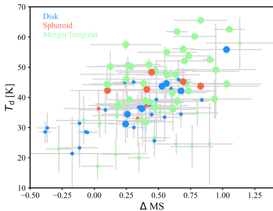
Figure 14. Same as Figure 13b. Colors are the morphological classes from Chang et al. (2018). The sizes of the data points indicate L_{\text{IR}} , where big circles are sources with L_{\text{IR}} > 10^{12} L_{\odot} . Sources that have merger or irregular features tend to have warmer T_d for a fixed \Delta MS . This finding further supports the scenario that mergers lead to an increase in T_d .
