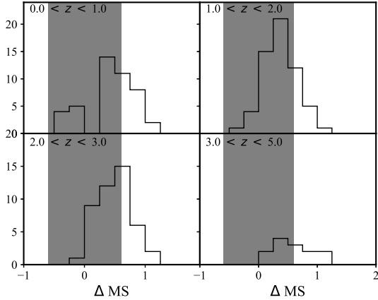
Figure 11. Histogram of main-sequence deviation \Delta MS of our sample in different redshift bins. The shaded areas show the range of 3\sigma scatter ( \pm 0.6 dex) of the Speagle et al. (2014) relations. A significant fraction of our sample, 58/162 ( 35_{-25}^{+32}\% ), can be classified as starburst galaxies.
