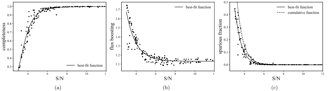
Figure A.1. (a) Completeness, (b) flux boosting, and (c) spurious source corrections from 200 source realizations as a function of S/N.
