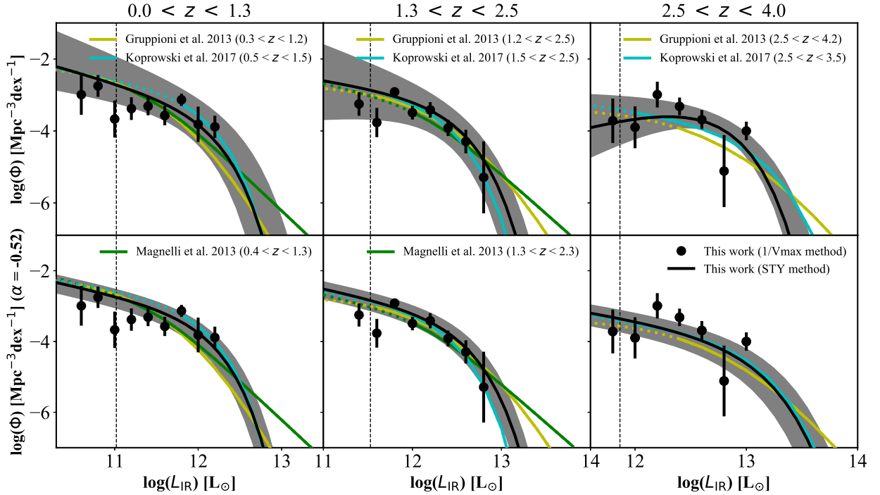
Figure 16. Upper panels: infrared LFs estimated using our 1/V_{\max} method (black points) and likelihood method (black curves) in three redshift bins. The uncertainties of the 1/V_{\max} LFs are calculated using the Poisson errors, while the errors of the likelihood LFs (dark shaded regions) are calculated as |\Delta\chi^2| \leq 2.3(\pm 1\sigma) . Lower panels: same as the upper panels, except that the likelihood LFs are estimated with a fixed \alpha of -0.5 \pm 0.7 and their corresponding errors are calculated as |\Delta\chi^2| \leq 1.0(\pm 1\sigma) . We also present the LFs from Herschel /PACS (Magnelli et al. 2013), PEP-HerMES/ Herschel (Gruppioni et al. 2013) and the JCMT 850- \mu\text{m} -selected sample (Koprowski et al. 2017). The dashed curves represent published LFs that are extrapolated beyond their detection limits. The black dashed vertical lines show the median detection limit of our L_{\text{IR}} values for the corresponding redshift bins.
