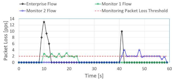
Fig. 6. Packet loss with switching module enabled
