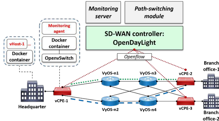
Fig. 1. SD-WAN architecture
