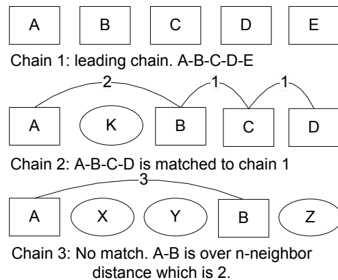
Figure 1: Definition of a similar code fragment
