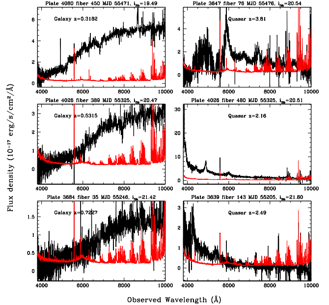
FIG. 4.— Examples of BOSS galaxy spectra (left) and quasar spectra (right), smoothed with a 3-pixel boxcar. In each panel, the black line is the spectrum and the red is the estimated error per pixel. The galaxy redshifts are 0.3182, 0.5315, and 0.7227 (top to bottom). The calcium H&K absorption features are near 5200, 6200, and 6800 \text{\AA} (top to bottom). Other noticeable features are the Mgb absorption line and [OII] and H \alpha emission lines. The quasar redshifts are 3.81, 2.16, and 2.49 (top to bottom). The Ly \alpha , CIV, and CIII] emission lines are identifiable features in these quasar spectra. The 2'' -fiber i -band magnitudes of the targets are listed above each panel.
