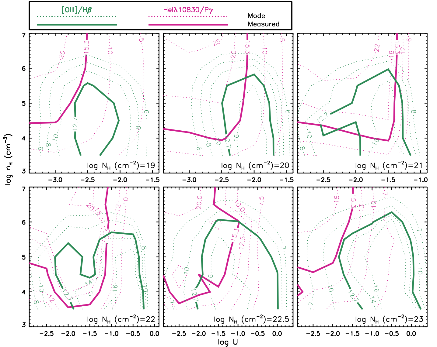
Figure 11. Photoionization models of the emission line outflow in J1634+2049 assuming solar abundances and dust free. Different panels are for models with different N_{\text{H}} . The green and violet dashed lines show the contours of line ratios of [\text{O III}]\lambda 5007/\text{H}\beta and \text{He I}\lambda 10830/\text{P}\gamma in (U, n_{\text{H}}) , respectively. The green and violet solid lines represent the locus of the measured upper limit for line ratios of [\text{O III}]\lambda 5007/\text{H}\beta and \text{He I}\lambda 10830/\text{P}\gamma , respectively. The closed region surrounded by the green and violet solid lines are the possible parameter space for the emission line outflow of J1634+2049.
