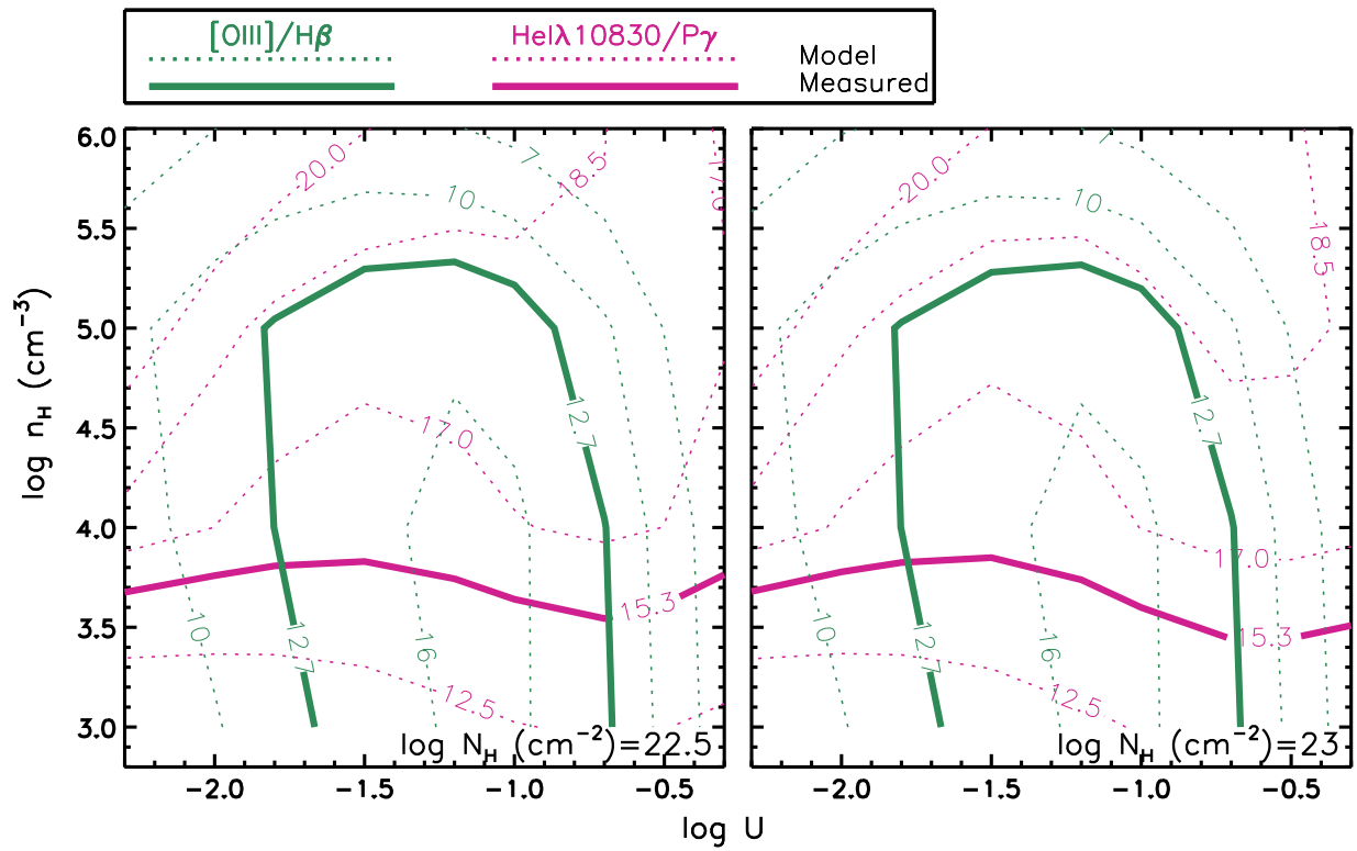
Figure 12. Dust models of the emission line outflow in J1634+2049. The emission line ratios are directly extracted from the best dust models of absorption line outflow. The symbols are the same as Figure 11.
