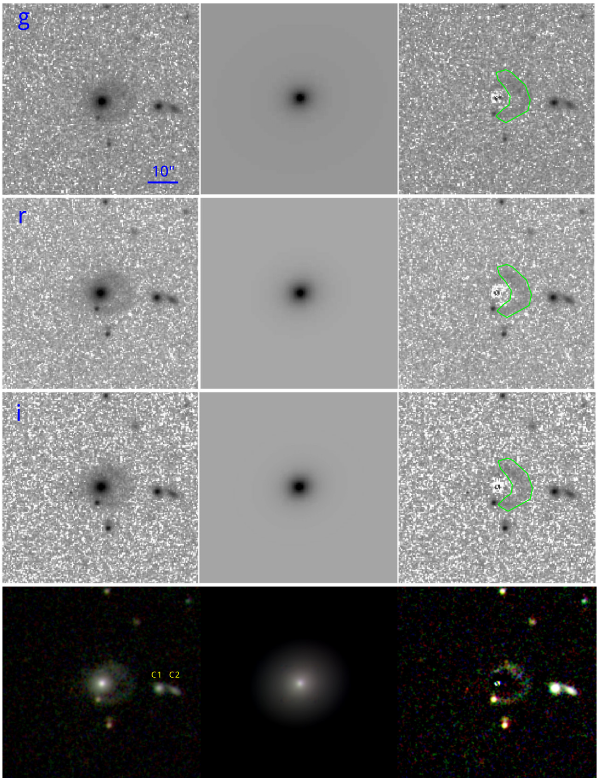
Figure 2. SDSS images of J1634+2049 and the 2D imaging decomposition by GALFIT. From top to bottom are SDSS g , r , and i bands, and the composite of the three bands, respectively. The left column shows the original image, the middle column shows the GALFIT model (PSF + Sérsic), and the right column shows the residual image. All images are oriented with north up and east to the left; the black line marks a scale of 10'' ( \sim 23.1 kpc). The green polygon denotes the ring region, which as well as the foreground stars has been masked out in GALFIT fitting.
