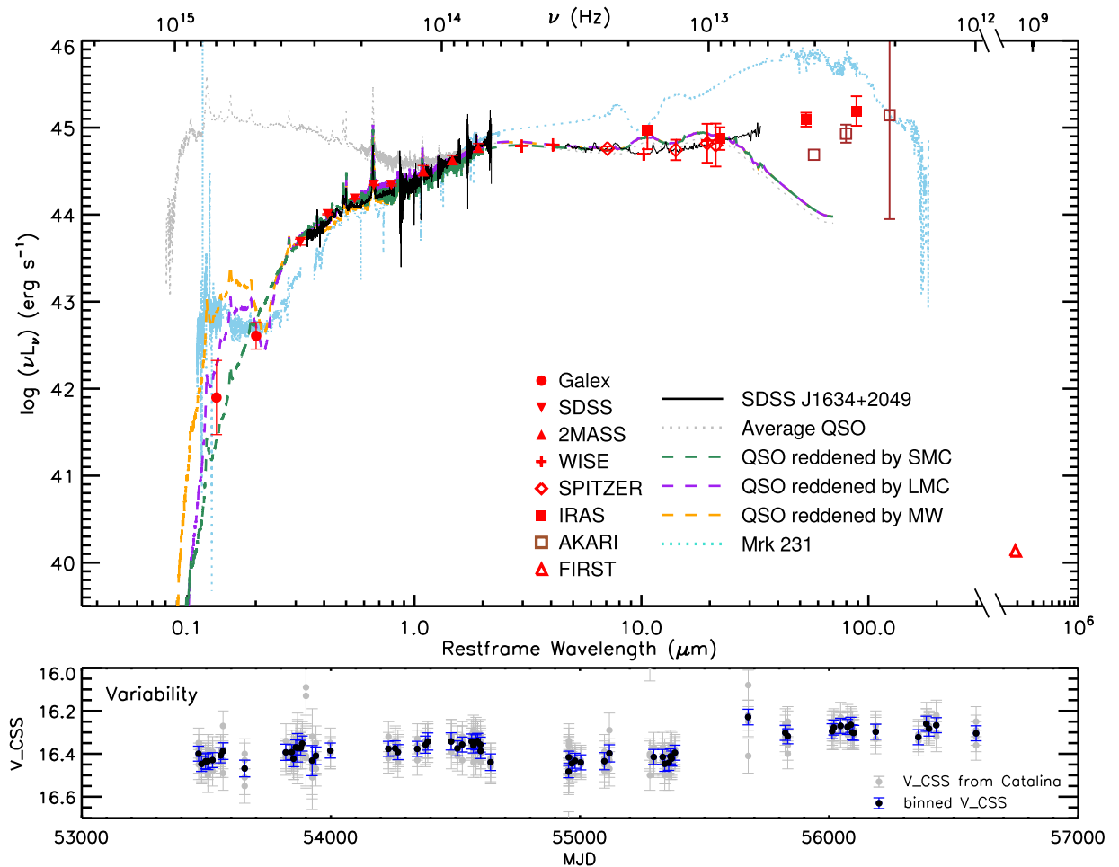
Figure 1. Top: the broadband spectral energy distribution of J1634+2049 constructed from non-simultaneous photometry data (red) and spectra, corrected for Galactic reddening and brought to the rest frame. The black solid lines are the SDSS spectrum, the NIR spectrum observed by P200 TripleSpec, and the Spitzer IRS spectrum. Overplotted for comparison is the average QSO spectrum (gray dotted line; see the text); the reddened versions of the average QSO spectrum by different extinction curves are denoted by the orange (MW), purple (LMC), and green (SMC) dashed lines. The light blue dotted line is the SED of Mrk 231, constructed from the multiband spectra scaled at \sim 2 \mu\text{m} . Bottom: the variability of the V band of J1634+2049. The raw data (gray dots) are taken from Catalina Survey with the binned version within every day plotted also (black dot).
