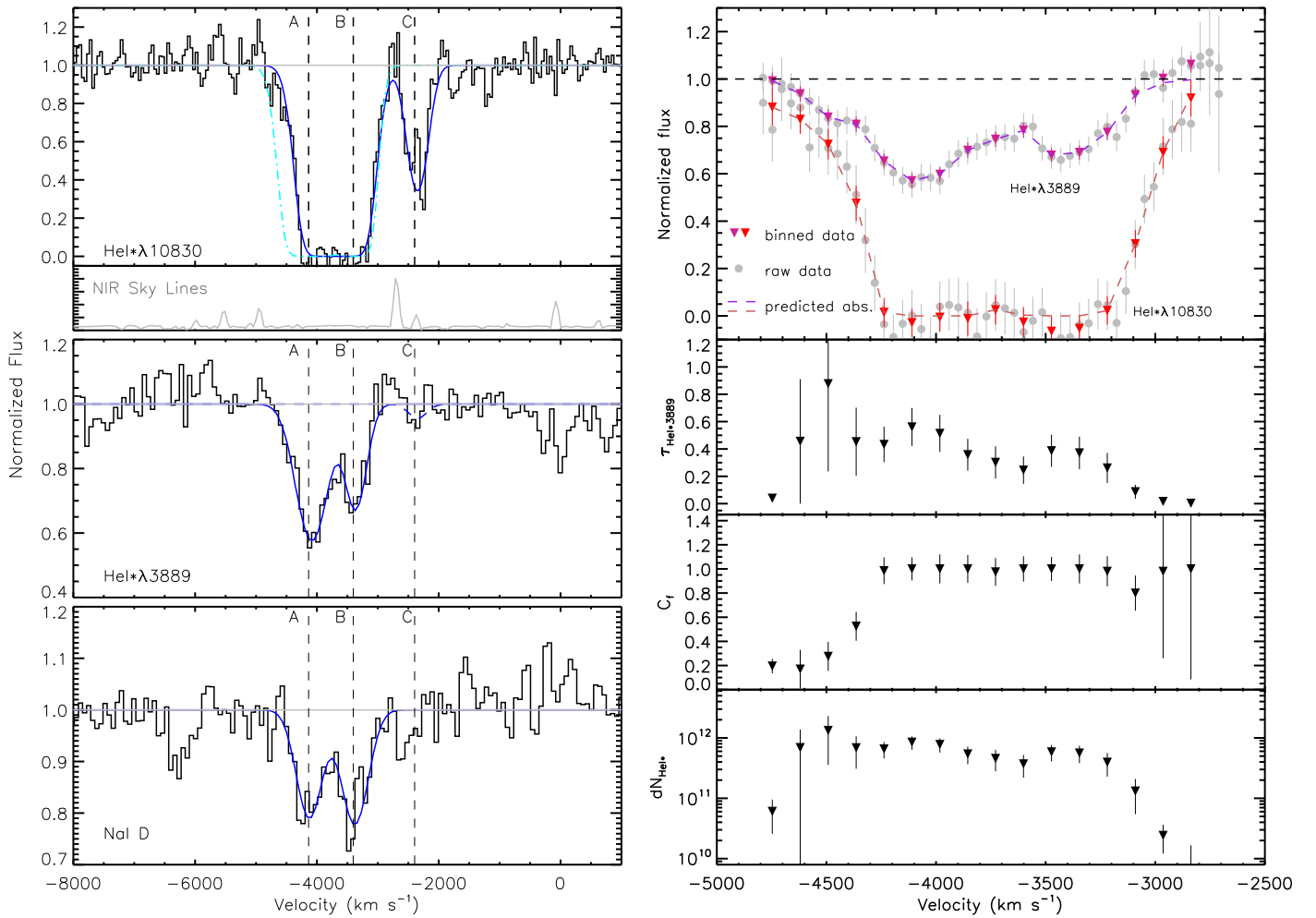
Figure 7. Left: demonstration of the absorption troughs in He I* \lambda\lambda 10830, 3889 and Na I D of J1634+2049, and the best fittings (in blue) by Voigt profile. The cyan lines in the upper panel show the predicted He I* \lambda 10830 profile derived from the He I* \lambda 3889 absorption line under the fully coverage assumption. Right: calculation results (top panel) of the He I* absorption lines of J1634+2049 using the partial-coverage model. The top panel shows the observed profiles (the gray dots) with \pm 1\sigma error bars of He I* \lambda\lambda 10830, 3889 the profiles binned by 3 pixels (the colored triangles), and the predicted profile from calculation (the dashed lines). The model parameters (the optical depth \tau_{\text{He I}^*\lambda 3889} , covering fraction ( C_I ), and column density ( dN_{\text{He I}^*} ) of the outflow) as a functions of velocity are shown in the other three panels.
