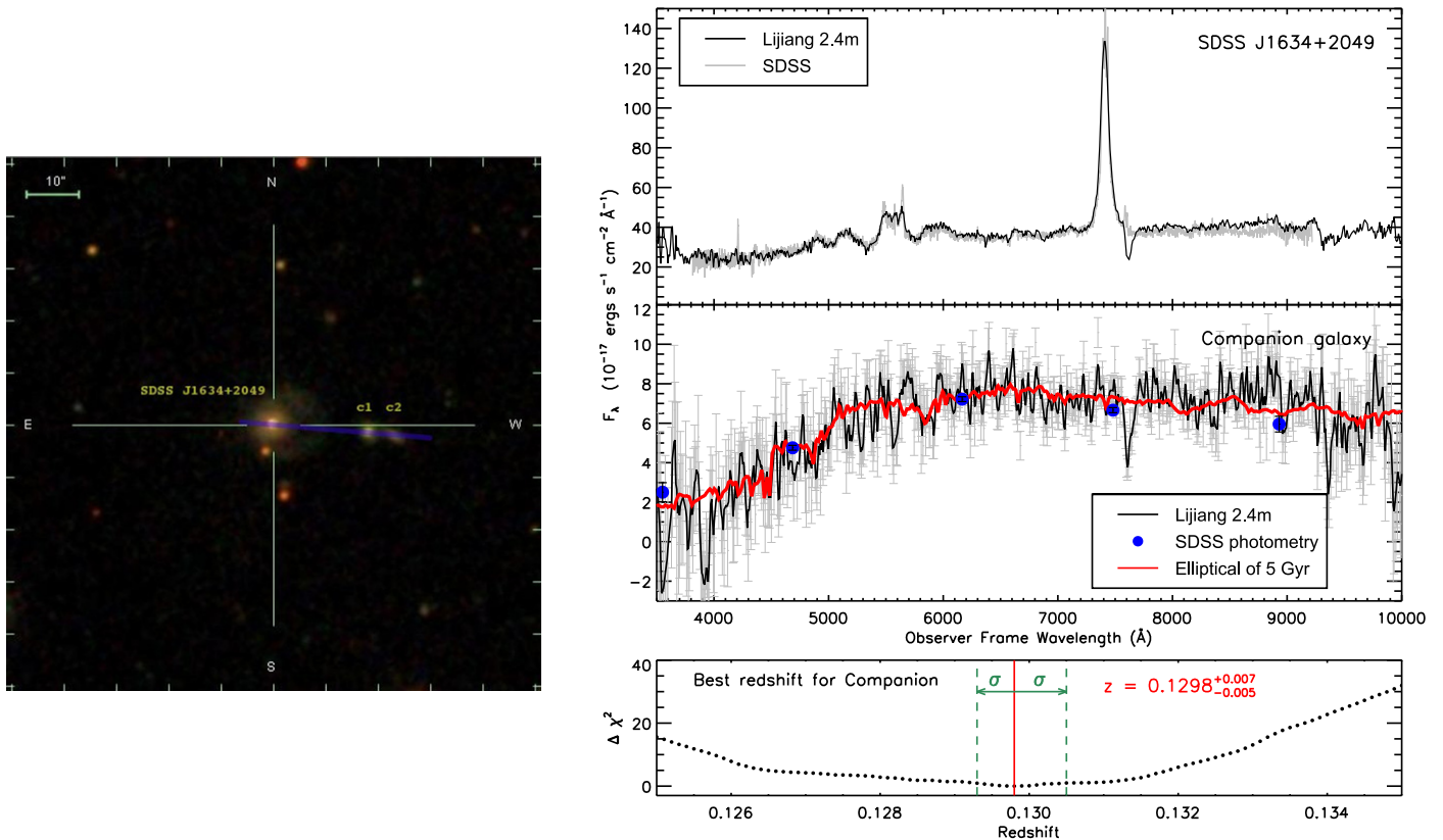
Figure 9. Left: SDSS image of J1634+2049 and its companion galaxy, C1. The PA = 86° slit position is displayed by a blue line. Right: the upper panel shows the Lijiang 2.4 m spectrum in the observer frame of J1634+2049 SDSS spectrum of J1634+2049 (the gray line in the upper panel) is displayed for a comparison. The middle panel displays the Lijiang 2.4 m spectrum of the companion galaxy C1. SDSS photometry of C1 are also plotted on the observed spectrum as a check. The red line represents a template of an elliptical of 5 Gyr, which is obtained from (Polletta et al. 2007). The lower panel shows the \Delta\chi^2 of the grid search of the redshift of C1. The best redshift is z = 0.1298_{-0.005}^{+0.007} .
