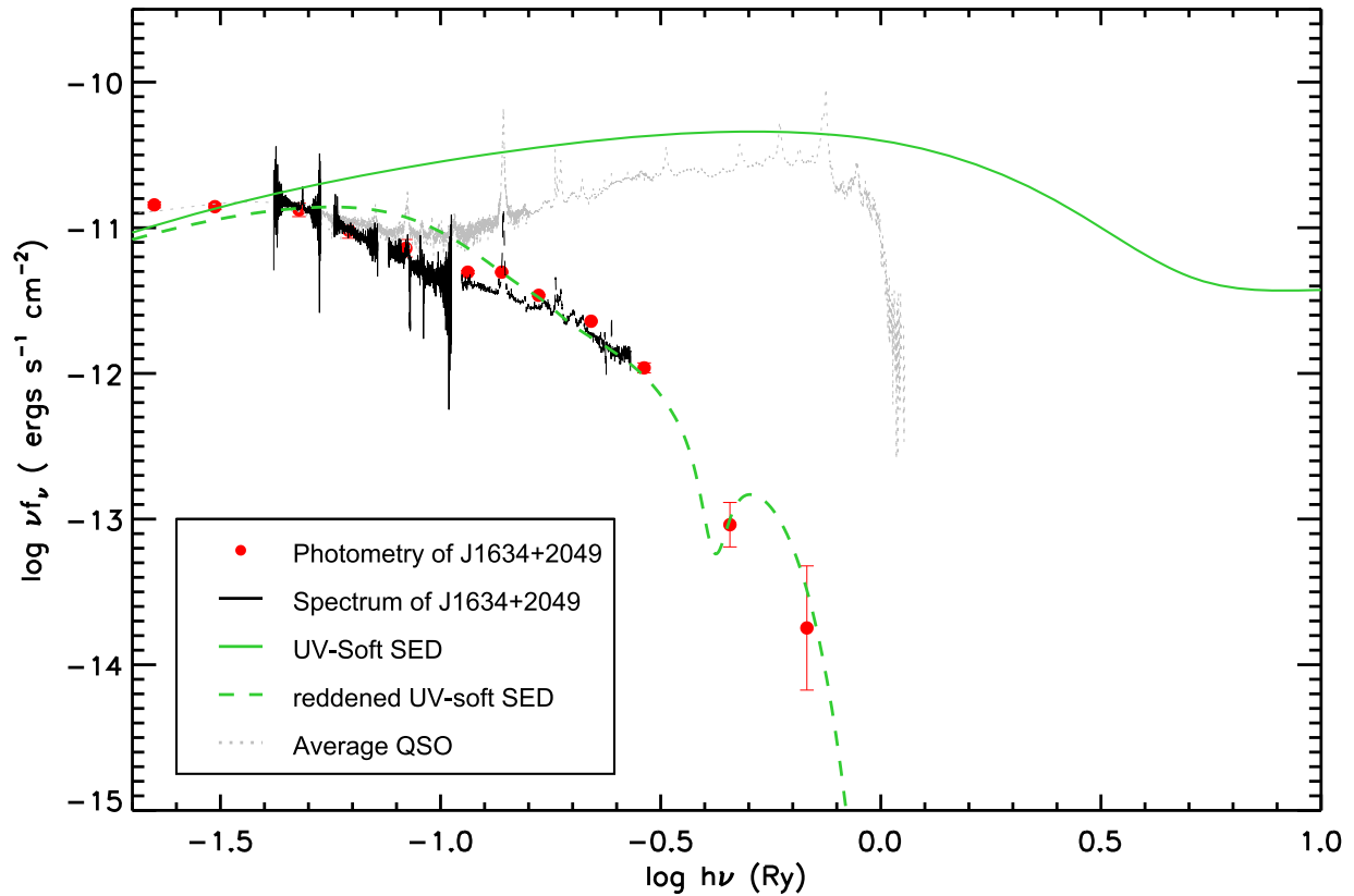
Figure 13. Observed spectrum (the black solid lines) and photometry data (the red dots) of J1634+2049. The green solid curve represents the UV-soft SED scaled to the observed flux at the WISE W1 band. The green dashed curve shows the UV-soft SED reddened with the LMC extinction curve. The gray dotted line is the average QSO spectrum as shown in Figure 1.
