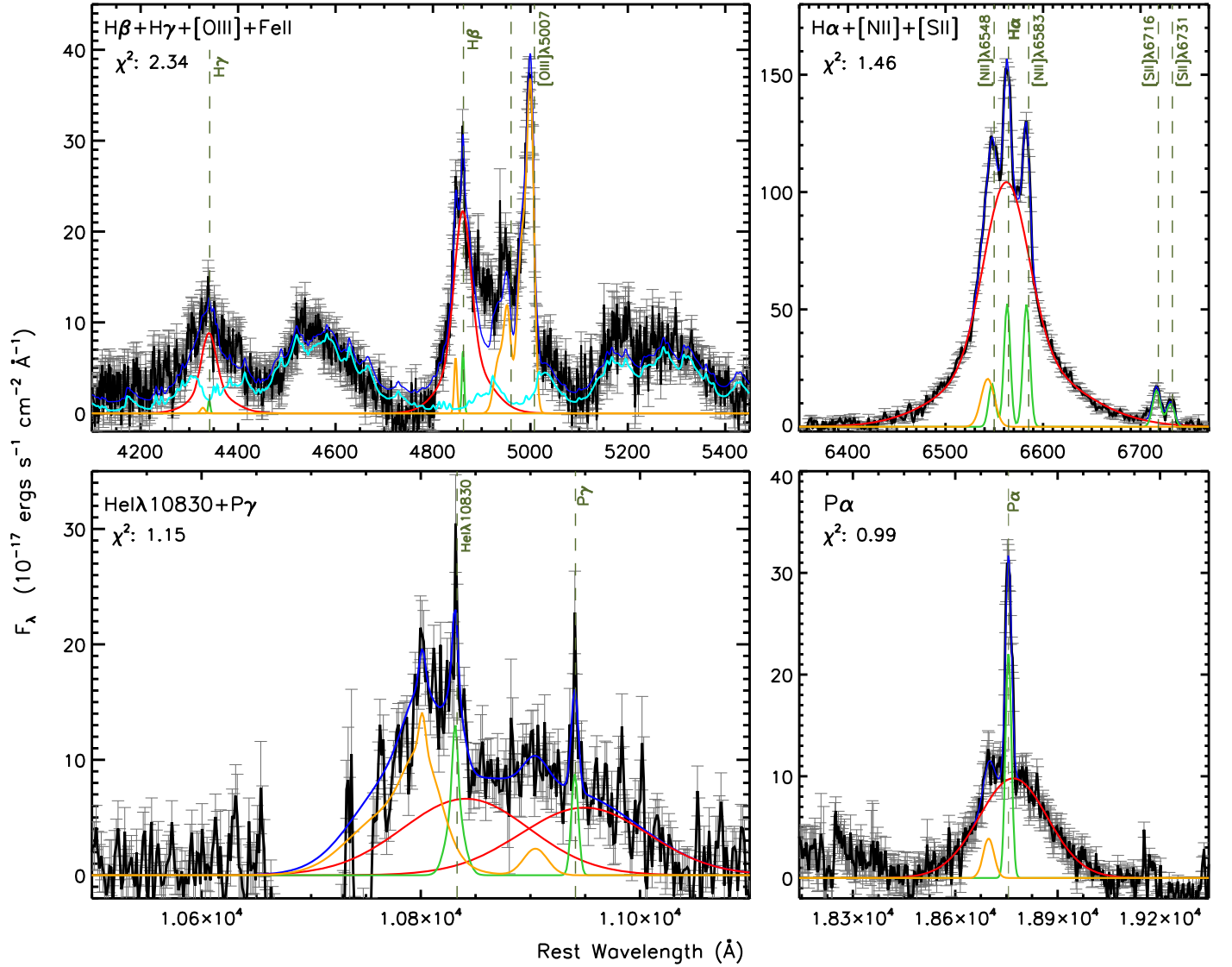
Figure 6. The best-fit models for H\beta + H\gamma + [O\ III] + Fe\ II region (upper left), H\alpha + [N\ II] + [S\ II] region (upper right), He\ I\lambda 10830 + P\gamma region (lower left), and P\alpha region (lower right). The blue solid line represents the total fit profile for each region. The red and green lines show the decomposed profiles of broad and narrow emission lines respectively. The orange line represents the blueshifted lines, and the cyan line represents optical Fe\ II multiplets.
