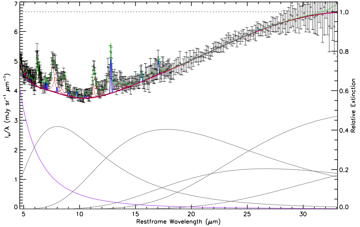
Figure 8. Best-fit decomposition of J1634+2049 from 5 to 33 \mu\text{m} (rest frame) from PAHFIT. Details of the model parameters can be found in Smith et al. (2007). The black circles with error bars show the observed data. The gray lines represent the thermal dust continuum components, the purple line shows the stellar continuum, and the red line shows the total (dust + stellar) continuum. The brown lines represent the PAH features and the blue lines show the atomic and molecular lines. All components are diminished by the fully mixed extinction, indicated by the dotted black lines, with the axis at the right. The green line is the full fitted model, plotted over the observed flux intensities and uncertainties.
