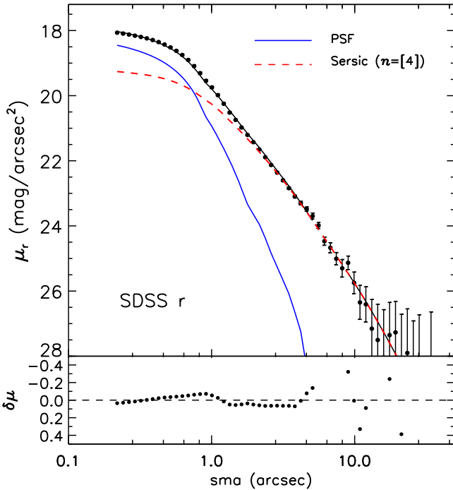
Figure 3. Top: one-dimensional representation of the two-component GALFIT model applied to the SDSS r image of J1634+2049: PSF for the nucleus (blue solid line) and n = 4 Sérsic function for the host galaxy (red dashed line). The sum of the two components is shown as the black solid line. The observed data are plotted as black dots with \pm 1\sigma error bars. Bottom: the residuals between the observed data and the best-fit model.
