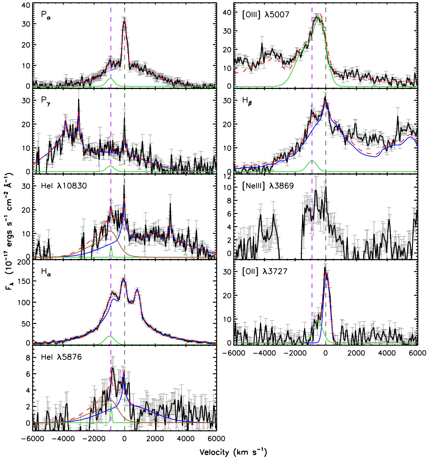
Figure 5. Demonstration of the profile of the various emission lines, particularly their blueshifted components (presumably caused by AGN outflow). Plotted are the observed spectra with continuum and Fe II emission subtracted (black line), the total fitted profile of each emission line (red dashed lines), the sum of the unblueshifted components of each line (blue lines), the narrow blueshifted component (green lines), and broad blueshifted component (brown lines). The purple and olive dashed vertical lines indicate -900 \text{ km s}^{-1} and 0 \text{ km s}^{-1} , respectively.
