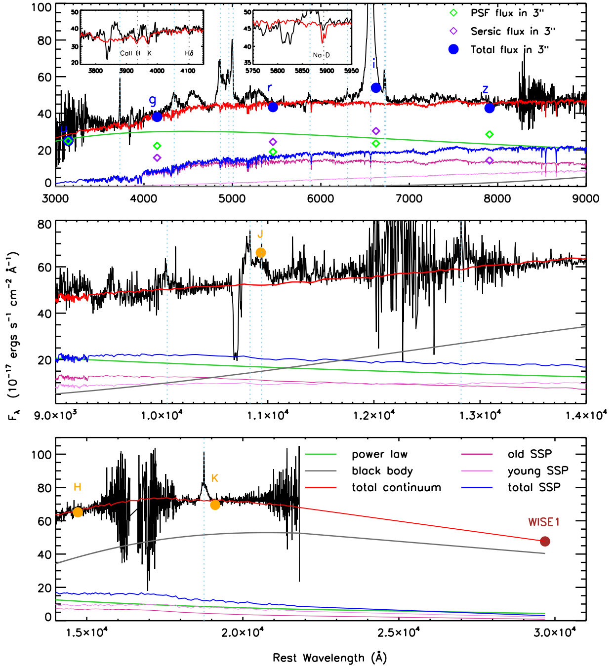
Figure 4. Detailed decomposition for continuum of J1634+2049 in the rest frame wavelength range from 3000 Å to 3 \mu\text{m} . The black solid line is the combined spectrum of SDSS (3350–8150 Å), DBSP (2900–9200 Å), and TripleSpec spectrum (8600 Å–2.2 \mu\text{m} ). The common parts of the three spectra were weighted by spectral signal-to-noise ratio (S/N). The blue solid dots are fluxes of u , g , r , i , and z bands in 3'' measured from SDSS images (see Section 2.3). The green and purple diamonds show the decomposition of PSF and Sérsic components in 3'' decomposed from SDSS images, respectively. The orange and brown dots are the photometry fluxes from 2MASS J , H , K , and WISE W1 bands. All the spectrum and photometry data are corrected for Galactic reddening and redshift. The green solid line represents the power-law component reddened by LMC extinction curve with E_{B-V} = 0.41 , and the gray line represents the blackbody continuum from hot dust (torus) with a temperature of 1394 K. The magenta line shows the continuum of the old stellar population (age \sim 9 Gyr), the violet line shows the heavily reddened continuum of the young stellar population (age \sim 127 Myr; E_{B-V} = 2.2 ), and the blue solid line shows the sum flux of the old and the young stellar population.
