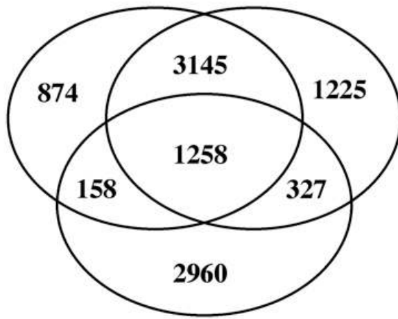
Figure S6.1: Venn diagram for three-way intron conservation comparison
