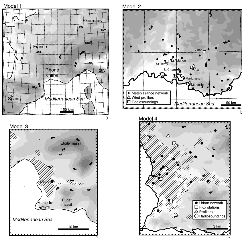
Fig. 1. Presentation of the four modeling domains with topography. For the two last models, the urbanized areas of Marseille are represented by hatchings. On models 2 and 4, are labeled the regional and urban observational networks, respectively
