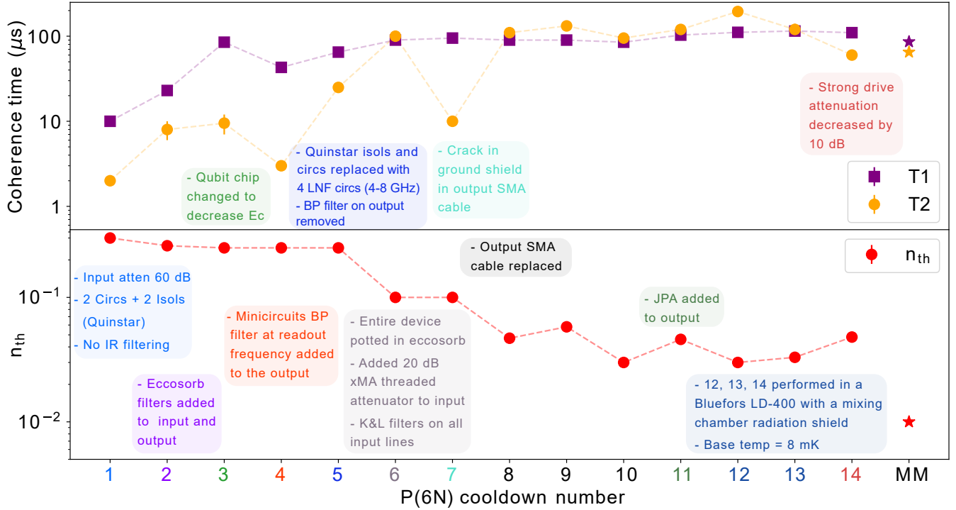
Supplementary Figure 4 | Evolution of (top) qubit coherence and (bottom) thermal population ( n_{\text{th}}^q ) for P(6N) over the course of 14 cooldowns. The primary changes that were made in each cooldown are listed in the legend (color coded with the cooldown number). The most important jumps to be noted are the reduction the qubit temperature from potting the device in IR absorber (6) and the improvement in the transmon T_2 in cooldown (5) from changes to the output line. These results were applied to the multimode device [MM2(5N5)], providing the coherence and temperature indicated by the \star .
