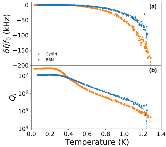
Supplementary Figure 3 | (a) The change in the TM_{011} mode frequency of the cylindrical flute cavity [C(6N)], and the TE_{101} mode of the rectangular pan-pipe cavity [R(6N)], as a function of temperature. (b) The corresponding internal quality factors as a function of temperature. The fits (dashed lines) give T_c \sim 1.31\text{K} and 1.25\text{K} for the C(6N) and R(6N) cavity, respectively. From the frequency fits, we can extract the London penetration lengths for both cavities, giving values of 235 \pm 3 \text{ nm} and 37.6 \pm 0.9 \text{ nm} , respectively.
