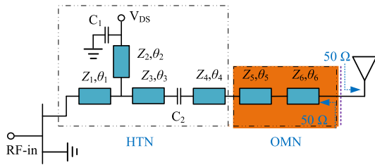
FIGURE 2. Schematic of a conventional AIA with a slot antenna.
