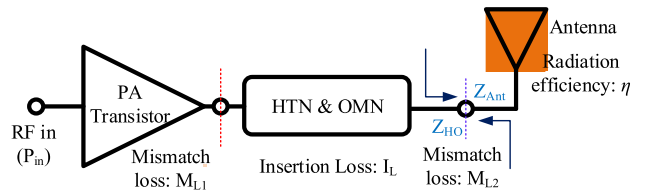
FIGURE 1. Conventional cascaded design of an AIA.
