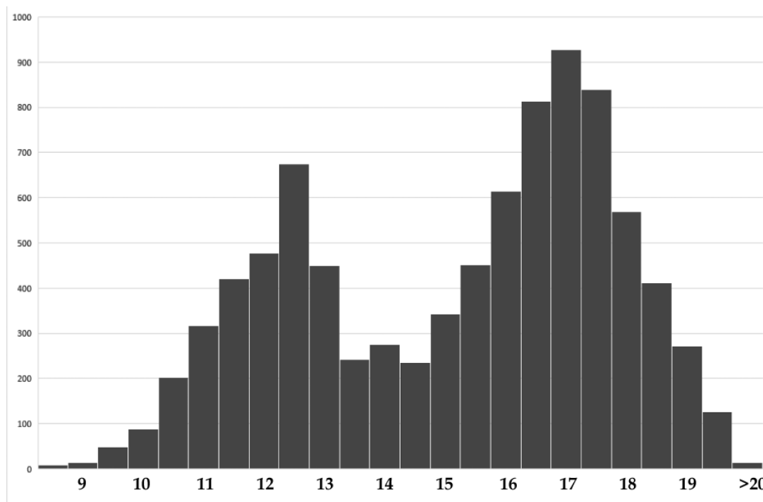
Figure 7. Distribution of objects in the ISON database by the average reduced brightness (vertical axis – number of objects, horizontal – brightness in magnitudes).
