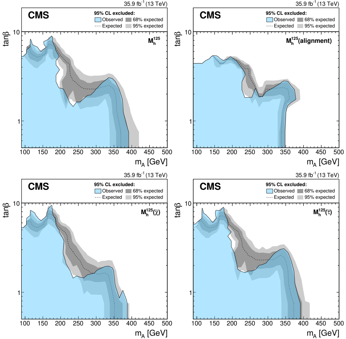
Figure 9. Expected and observed 95% CL upper limits on \tan\beta as a function of m_A for the M_h^{125} (upper left), M_h^{125} (alignment) (upper right), M_h^{125}(\tilde{\chi}) (lower left), and M_h^{125}(\tilde{\tau}) (lower right) scenarios. The expected limit is shown as a dashed black line while the dark and light gray bands indicate the 68 and 95% CL uncertainties, respectively. The observed exclusion contour is indicated by the blue area.
