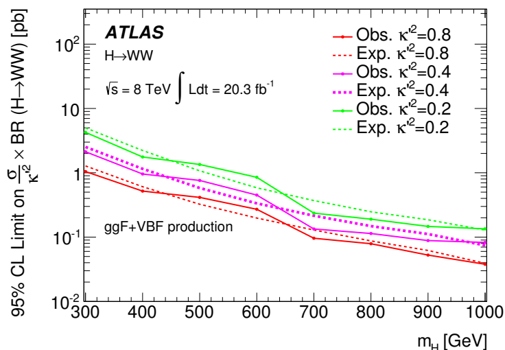
Figure 16. 95% CL upper limits in the intermediate-width scenario from the combination of the H \rightarrow WW \rightarrow l\nu l\nu and H \rightarrow WW \rightarrow lvqq final states. Limits are set on \frac{\sigma_H}{\kappa^2} \times \text{BR}(H \rightarrow WW) for a heavy scalar resonance with a width in the range 0.2\Gamma_{H,\text{SM}} \leq \Gamma_H \leq 0.8\Gamma_{H,\text{SM}} . The ggF and VBF production modes have been combined.
