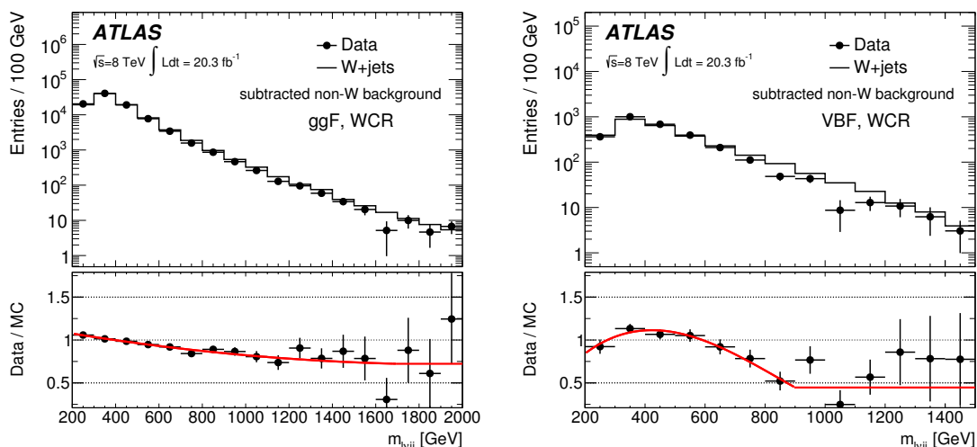
Figure 3. Data and Monte Carlo comparison of the shape of the invariant mass of the WW system m_{l\nu jj} in the ggF (left) and VBF (right) WCRs after the m_H = 300 GeV selection for the H \rightarrow WW \rightarrow l\nu qq analysis. All the lepton flavour and charge categories are summed together. To isolate the effects of W +jets background modelling, other contributions (top, diboson, Z +jets, multijet) are subtracted from the data. The Monte Carlo distributions are normalised to the remaining data. The ratio of the data to the Monte Carlo distribution is shown in the bottom panel, along with a red line showing the resulting weights that are applied to correct the Monte Carlo predictions in the rest of the analysis.
