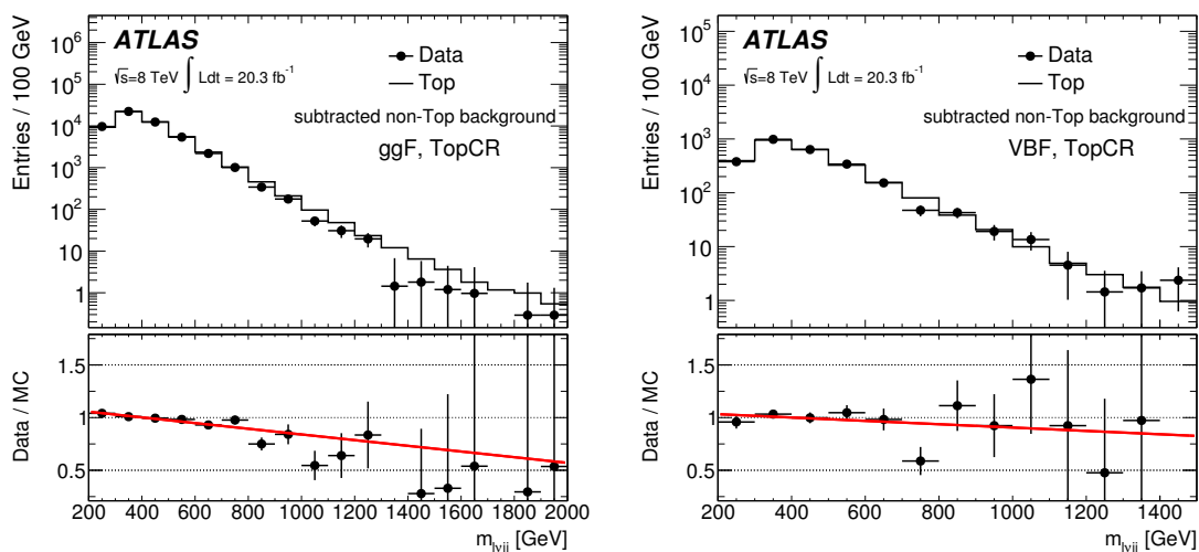
Figure 4. Data and Monte Carlo comparison of the shape of the invariant mass of the WW system m_{l\nu jj} in the ggF (left) and VBF (right) TopCRs after the m_H = 300 GeV selection for the H \rightarrow WW \rightarrow l\nu qq analysis. All the lepton flavour and charge categories are summed together. To isolate the effects of top-quark background modelling, other contributions ( W +jets, diboson, Z +jets, multijet) are subtracted from the data. The Monte Carlo distributions are normalised to the remaining data. The ratio of the data to the Monte Carlo distribution is shown in the bottom panel, along with a red line showing the resulting weights that are applied to correct the Monte Carlo predictions in the rest of the analysis.
